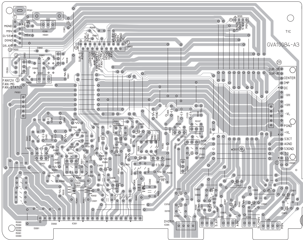
(Amplifier board 1)
