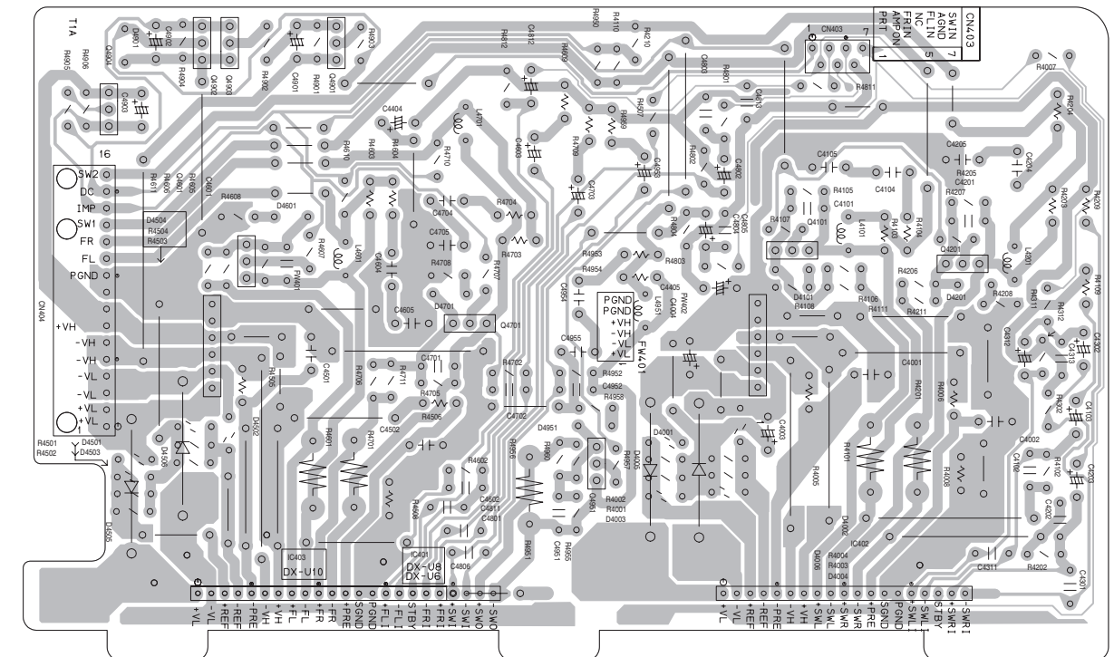
(Amplifier 2 board)
