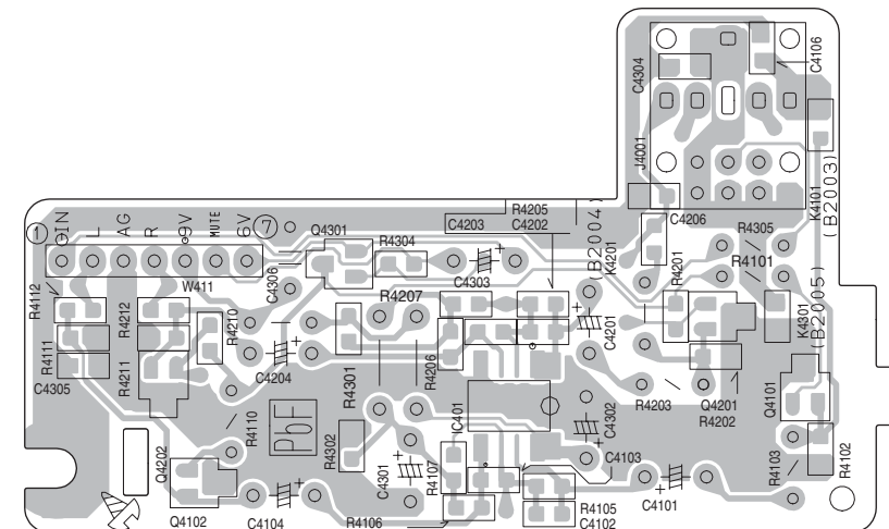
(Headphone board)
