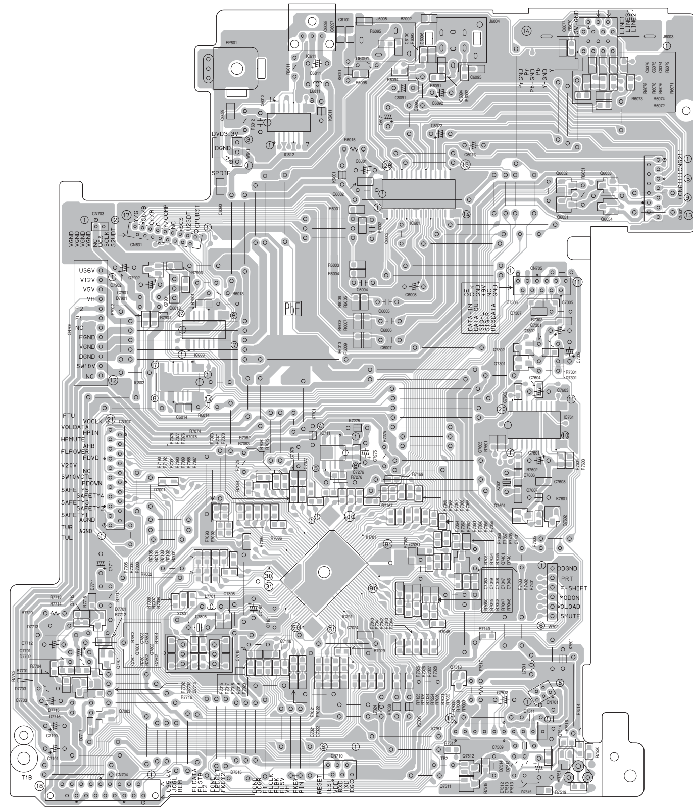
(Micom board)
