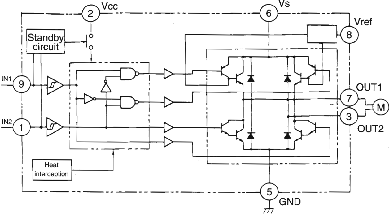
1.Block Diagram
