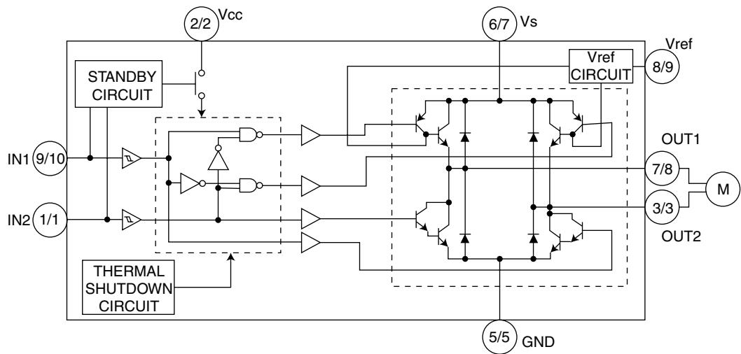
3. Block diagram
