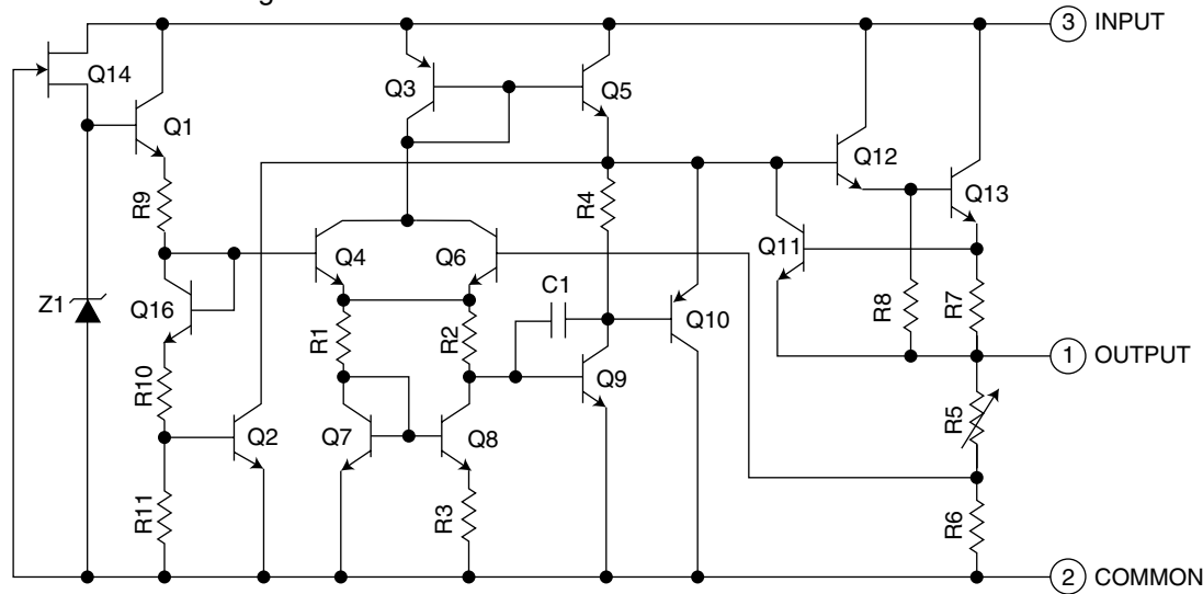
2. Block diagram
