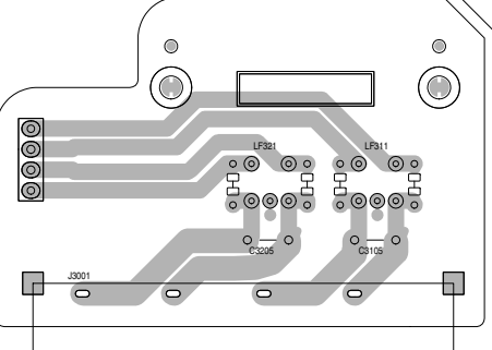
■ Speaker jack board
