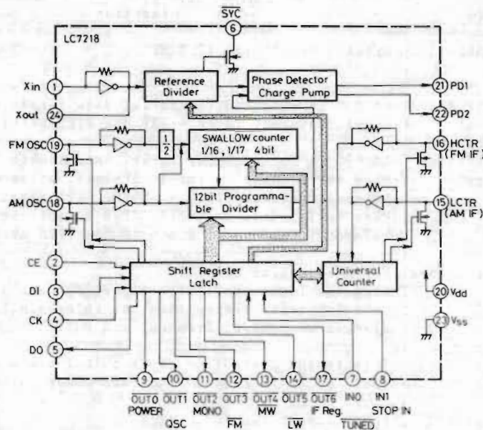
IC102 : LC7218 (PLL Synthesizer)
