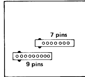
Top View of TAC-406
