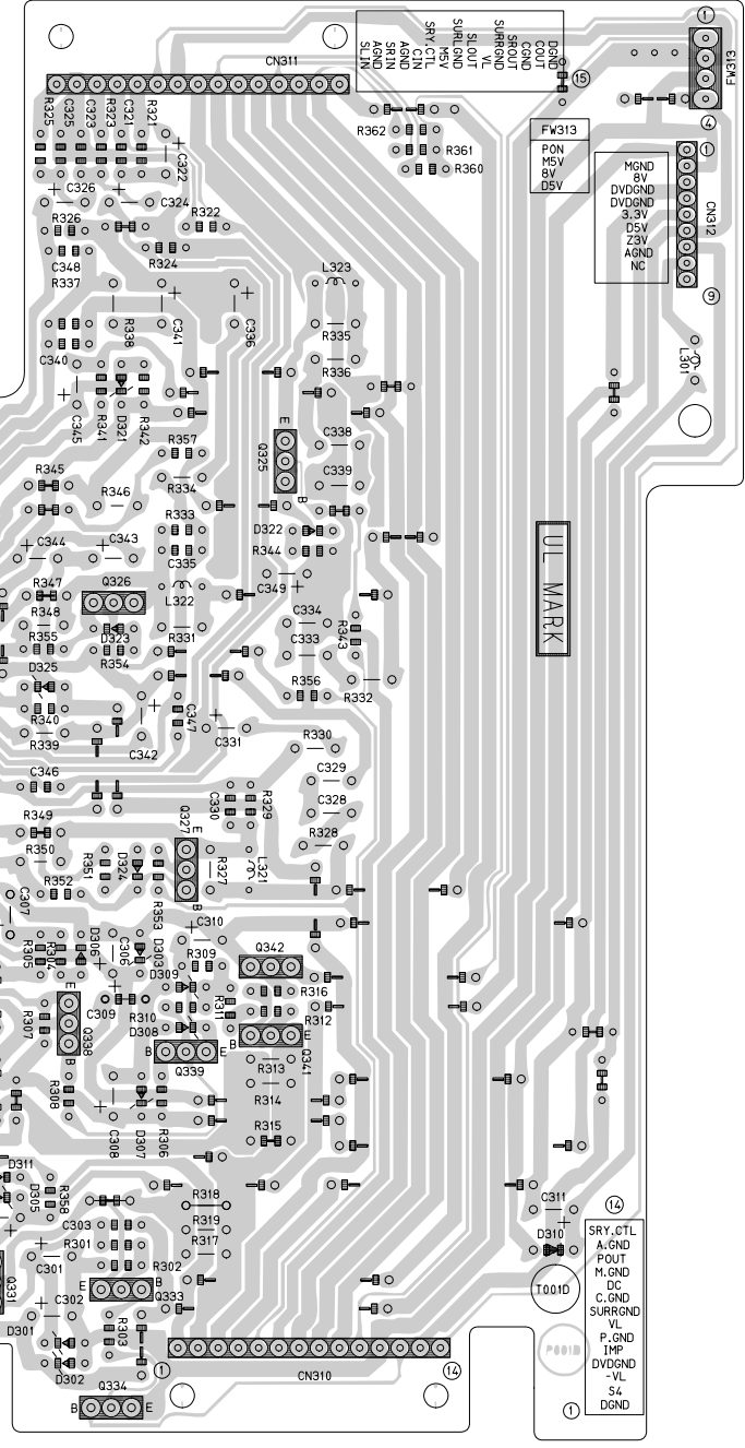
Amplifier board (1)
