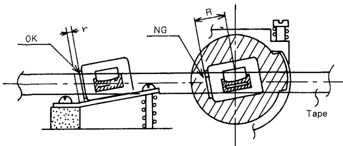
Fig. 21 Tape guide deviated
