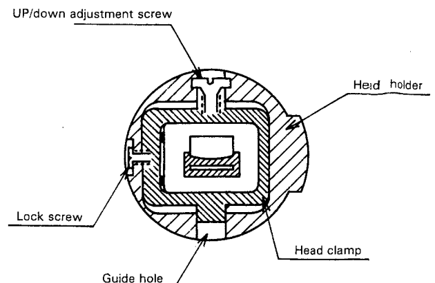
Fig. 22 Head up/down adjustment mechanism
