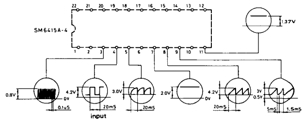
Fig. 21 Waveforms (Pin 1 through Pin 11)
