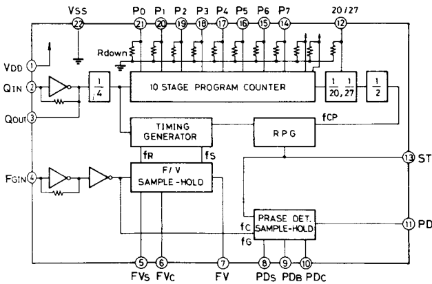
Fig. 19 Block Diagram
