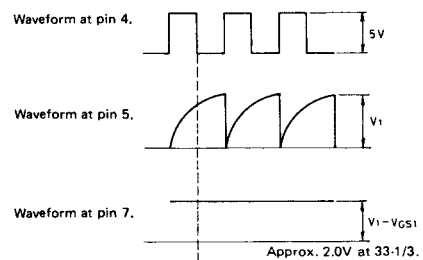
Fig. 22 Waveforms (F/V and P/D)
