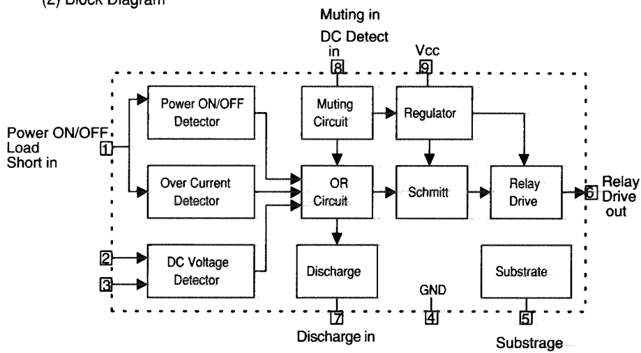
(2) Block Diagram
