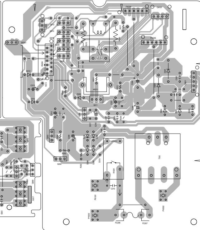
Power supply board
