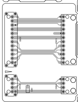
Relay board (tuner)
