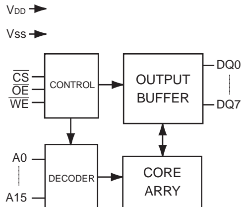
2. Block diagram
