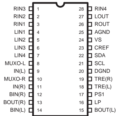
1. Terminal layout
