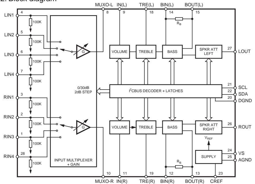
2. Block diagram
