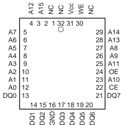
1. Pin layout
