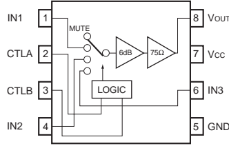
1. Block diagram
