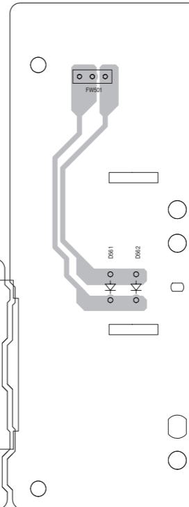
(LED board)
