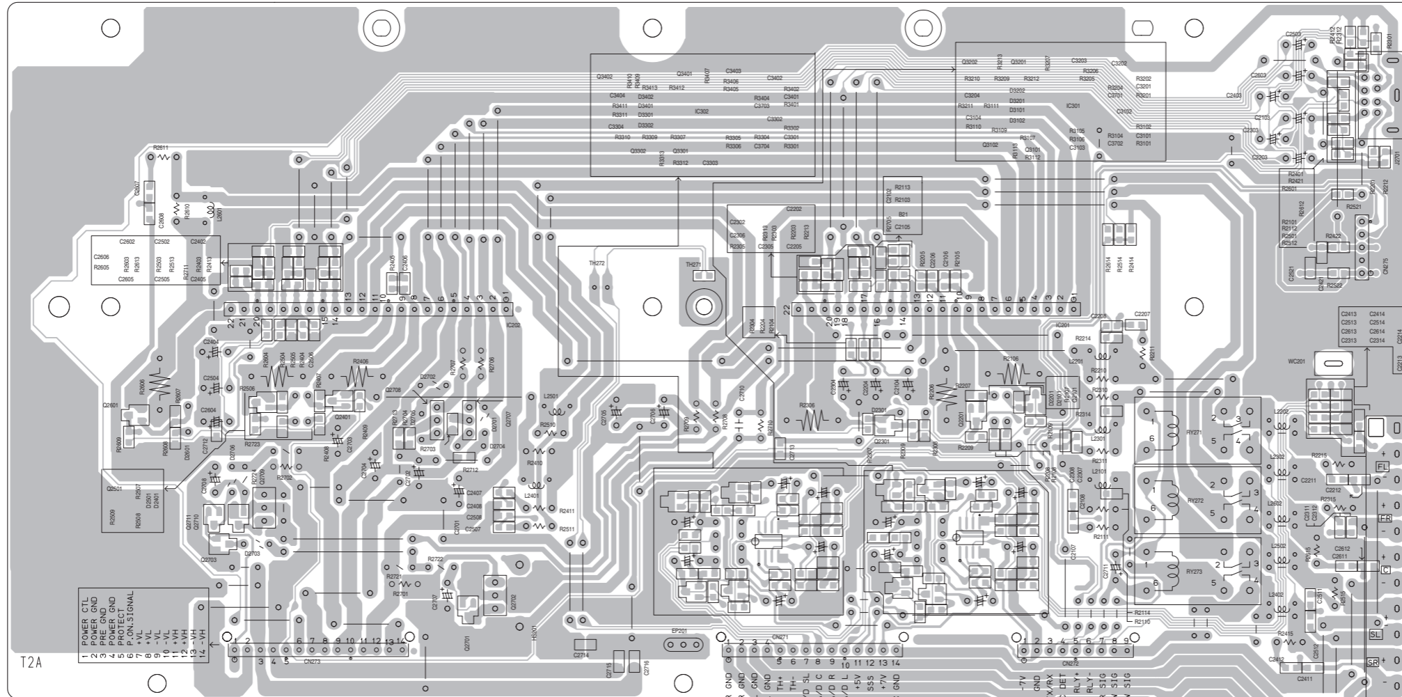
(Amp. board)
