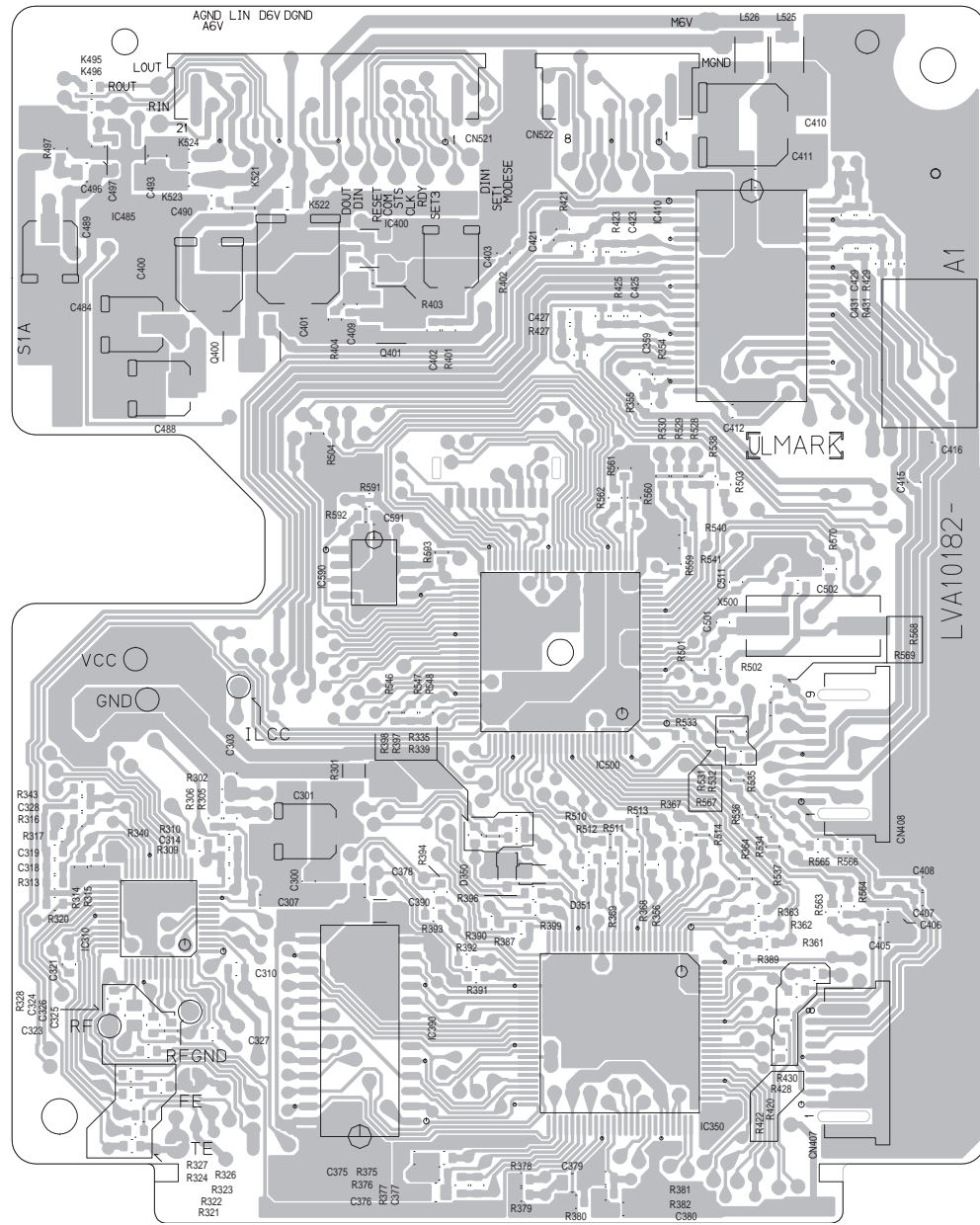
■ MD servo board (Forward side)
