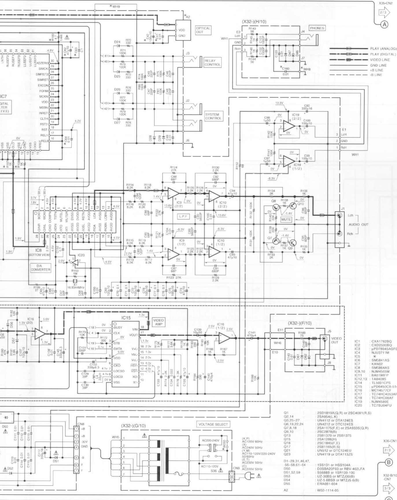
DP-R5080/R6080/R8080V(K)(1/3)
