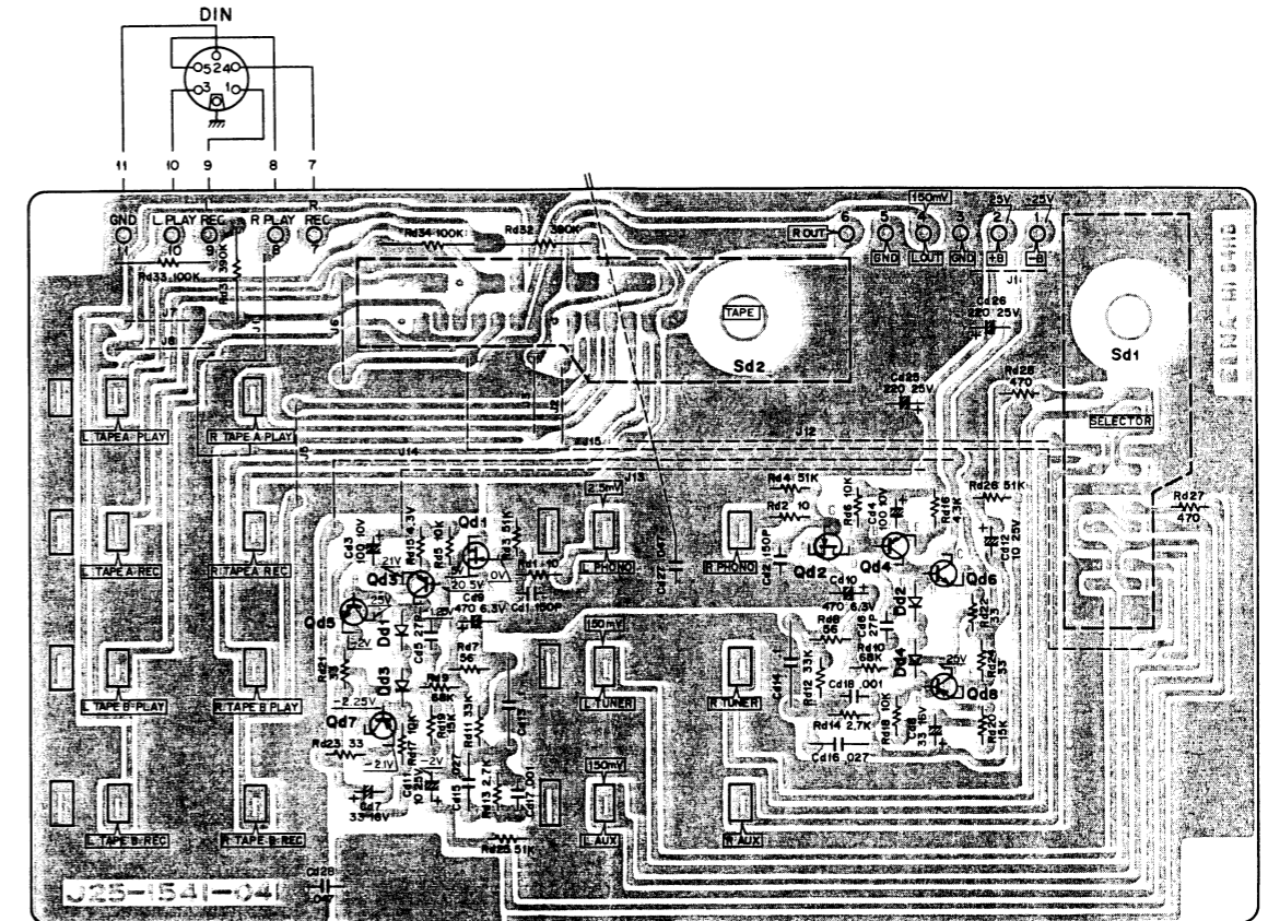
Qd1, 2: 2SK117 (O) or (Y) or (GR) or 2SK68A (K) or (L) or (M), Qd3, 4, 7, 8: 2SA640 (E) or (F) or 2SA841 (GR) or (BL), Qd5, 6: 2SC945 (P) or (Q) or (R) Dd1 ~ 4: 1S1555 or 1S2076
