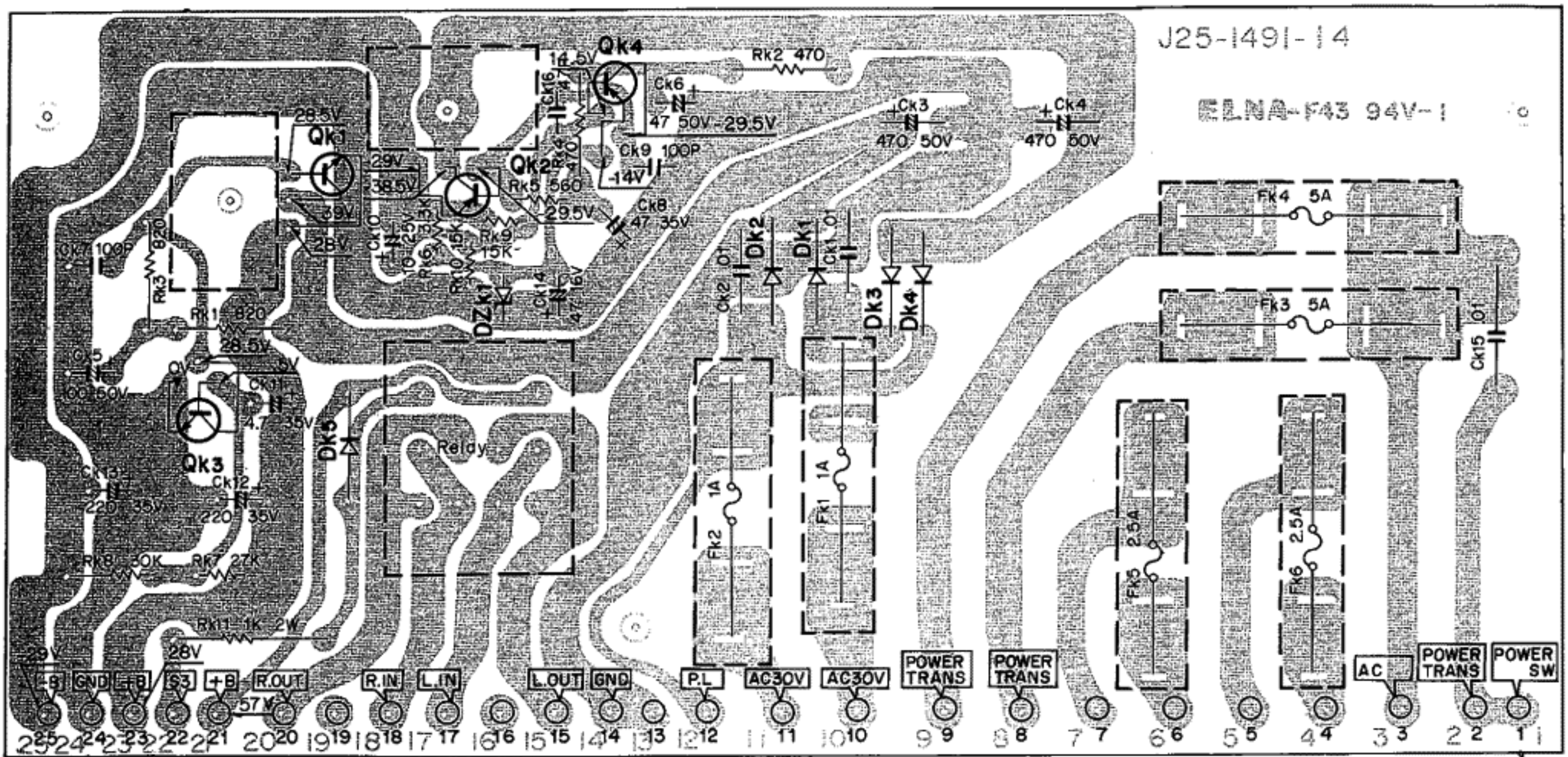
Qk1:2SC1983, Qk2:2SA755 (B) or (C), Qk3:2SC945 (Q) or (P), Qk4:2SA673A (C) or (D), Dk1~5:W06B, Dzk1:YZ-140
