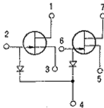
Schematic of μPA-63H
