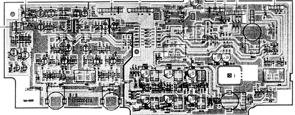
TONE AMP UNIT (X11-2222-71) (B/6) Component side view
