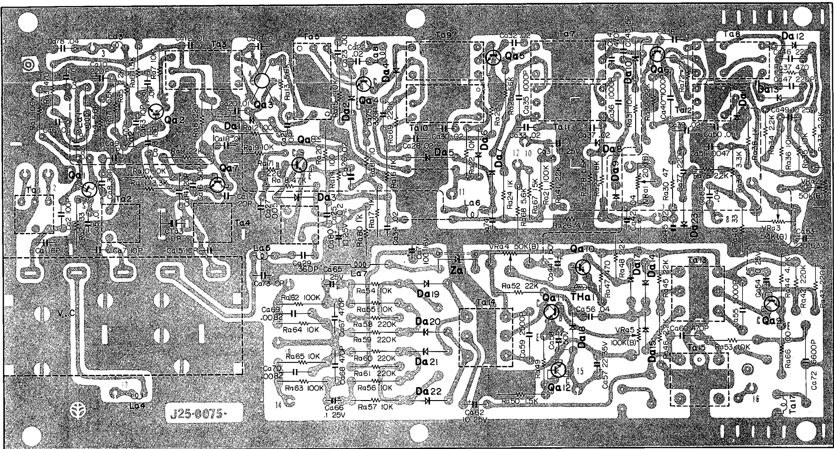
Qa1: 2SK19(GRorBL), Qa2,4-6: 2SC381(R), Qa3: CS5995(RorB), Qa7: 2SC785(R), Qa9: CS9014(B)or2SC458L(BorLC), Qa10: 2SB56A, Qa11: CS9014(C)or2SC458L, Qa12: 2SC734(Y) Da1,2,4~15, 17~23: IN60orIN34A, Za1: ZB1-14, THa1: SDT-1000Lor5T-41L
