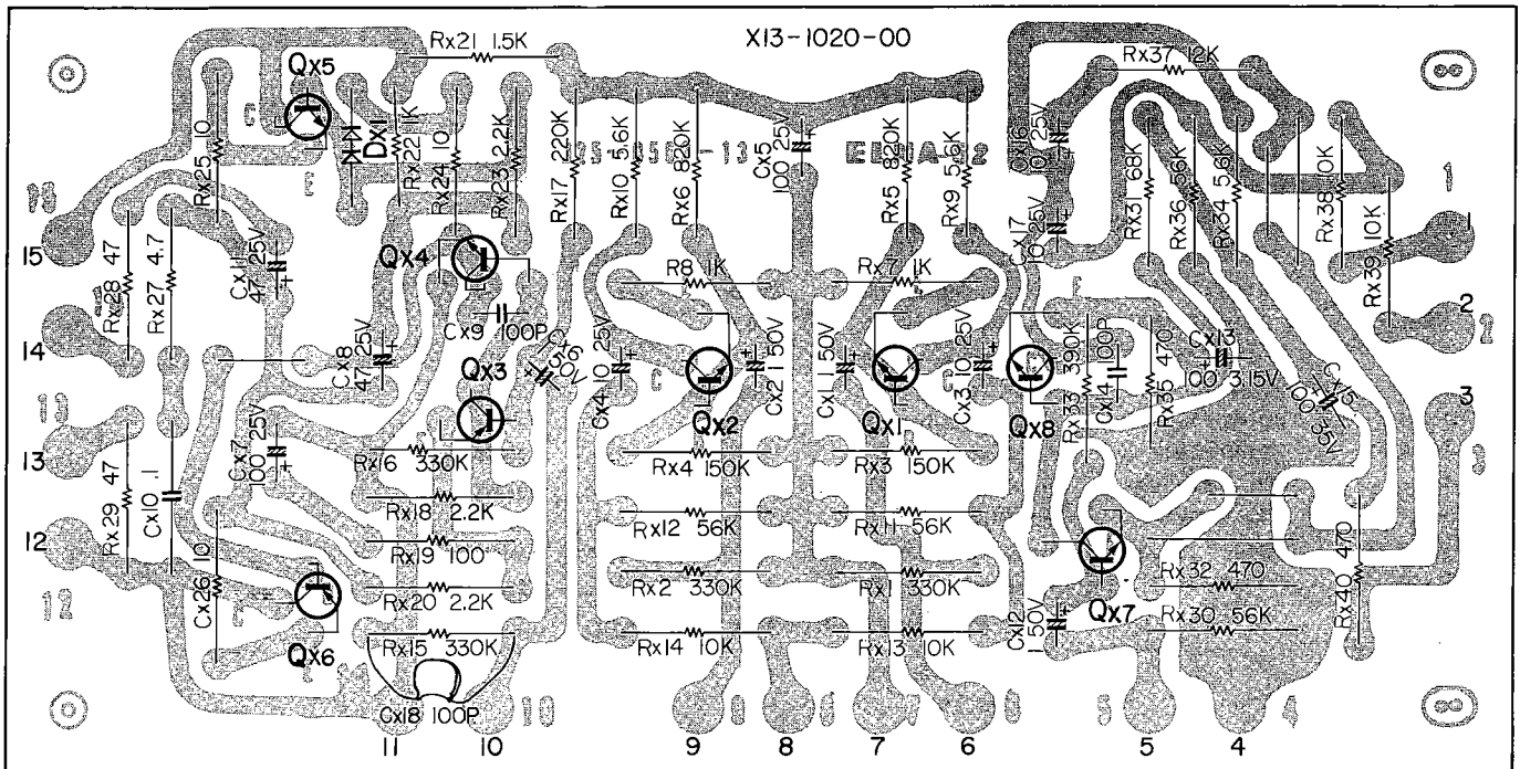
Qx1, 2, 7, 8: 2SC458LG (C) or (D), Qx3: 2SA493GR, Qx4: 2SC458 (C) or (D), Qx5: 2SC1213A (B) or (C), Qx6: 2SA673A (B) or (C) Dx1: MV-13
