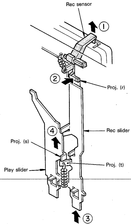
Fig. 11 RECORD operation (1)
