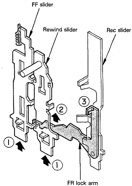
Fig. 13 RECORD operation (3)
