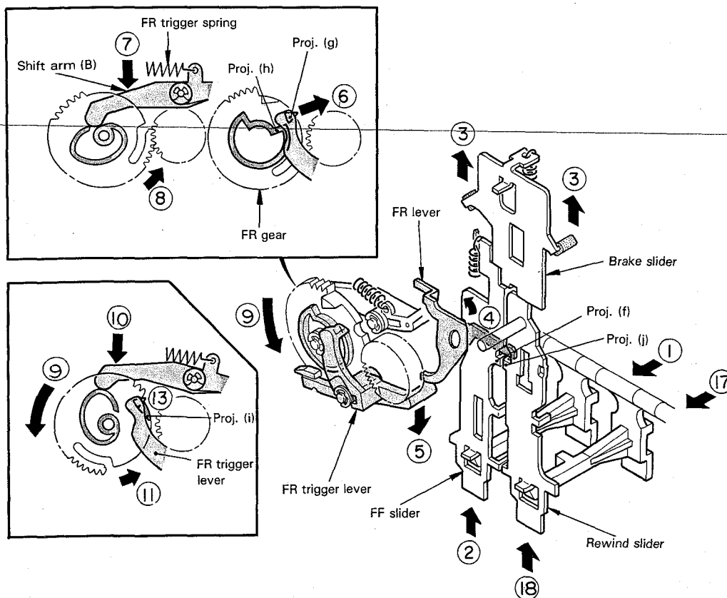
Fig. 6 FF operation (1)
