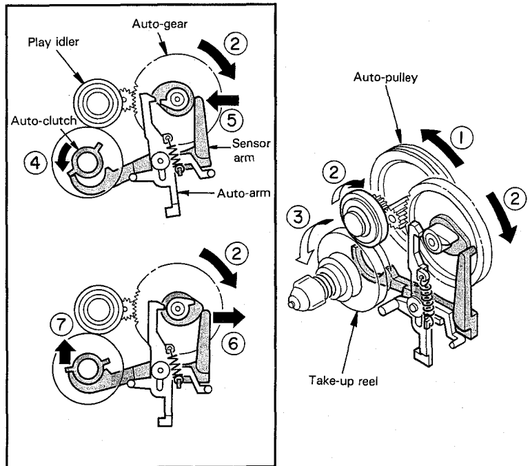
Fig. 14 AUTO-STOP operation (1)
