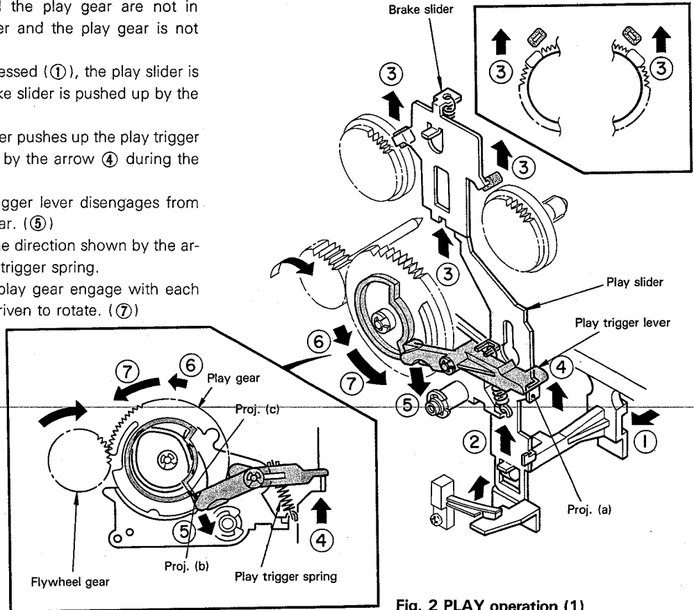
Fig. 2 PLAY operation (1)
