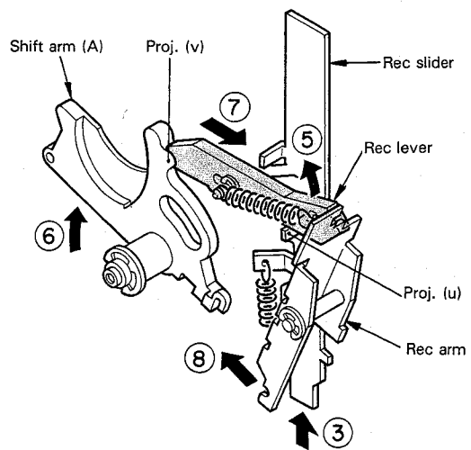
Fig. 12 RECORD operation (2)
