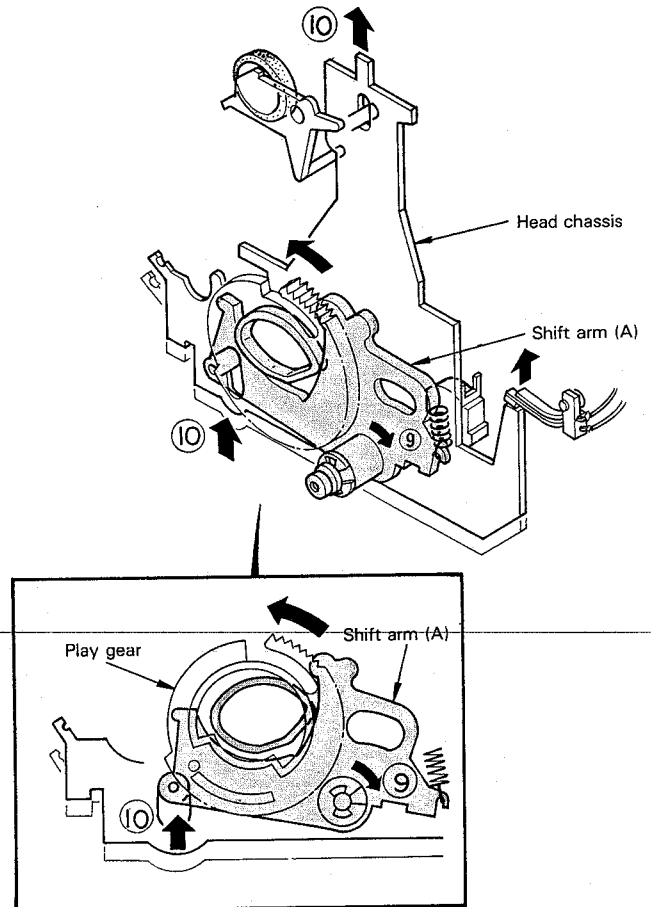
Fig. 4 PLAY operation (3)
