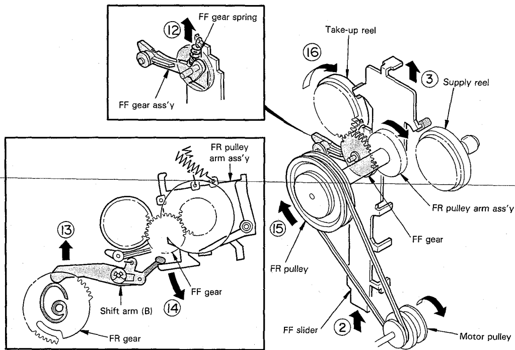
Fig. 7 FF operation (2)
