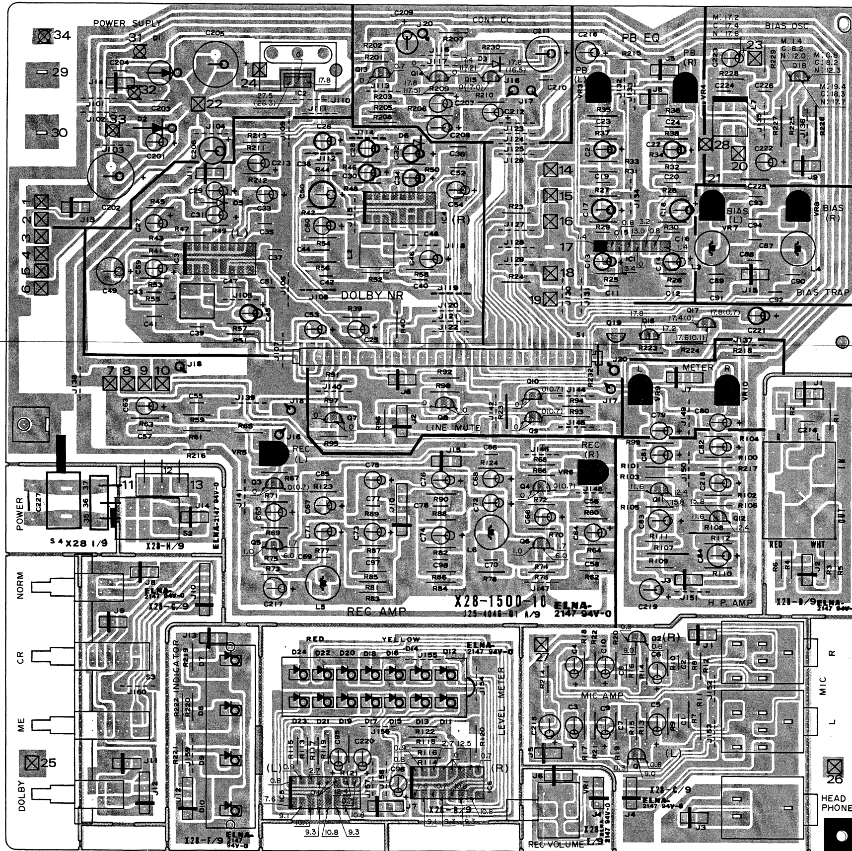
RECORD/PLAYBACK(X28-1500-10) Component side view
