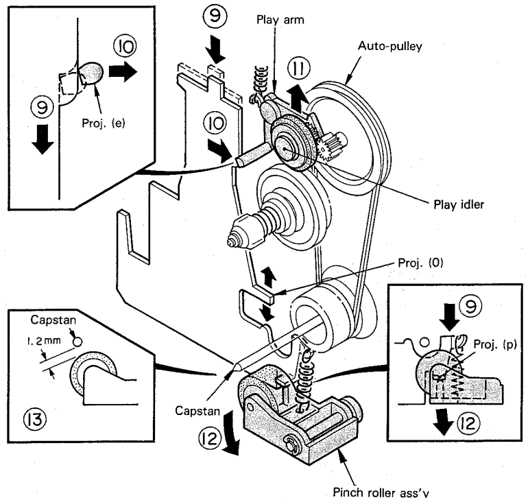
Fig. 10 PAUSE operation (2)
