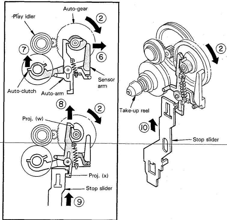
Fig. 15 AUTO-STOP operation (2)
