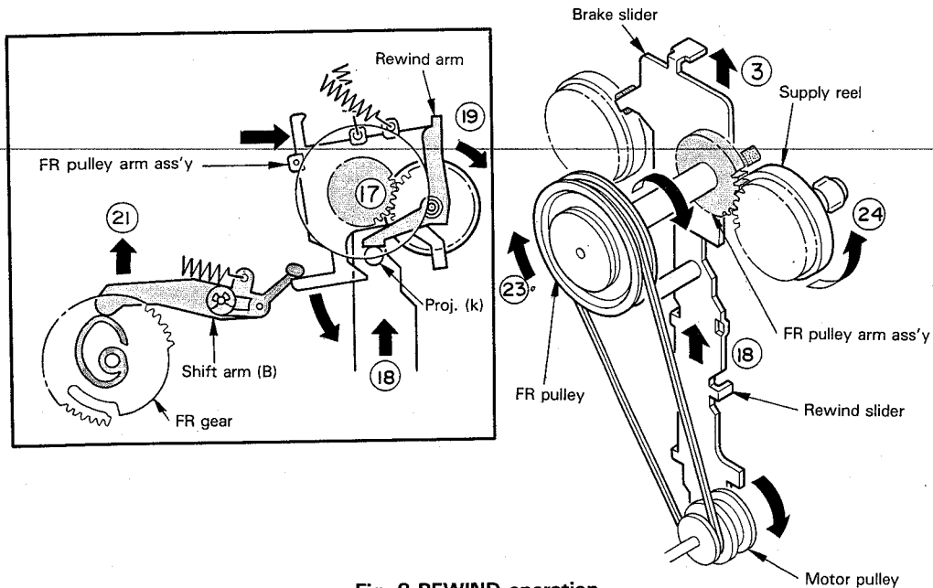
Fig. 8 REWIND operation
