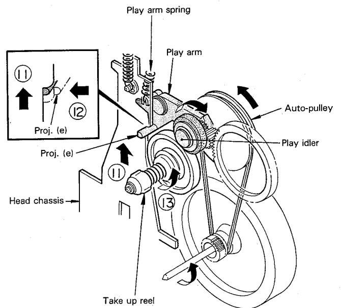
Fig. 5 PLAY operation (4)
