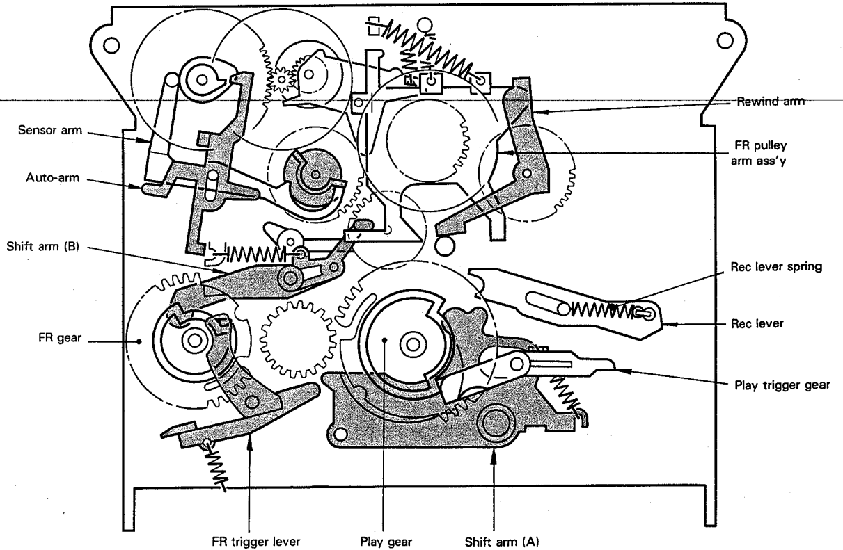
Fig. 1 Mechanism rear view
