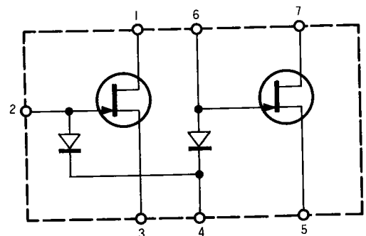
< Fig. 5 \mu PA-63H Interior >
