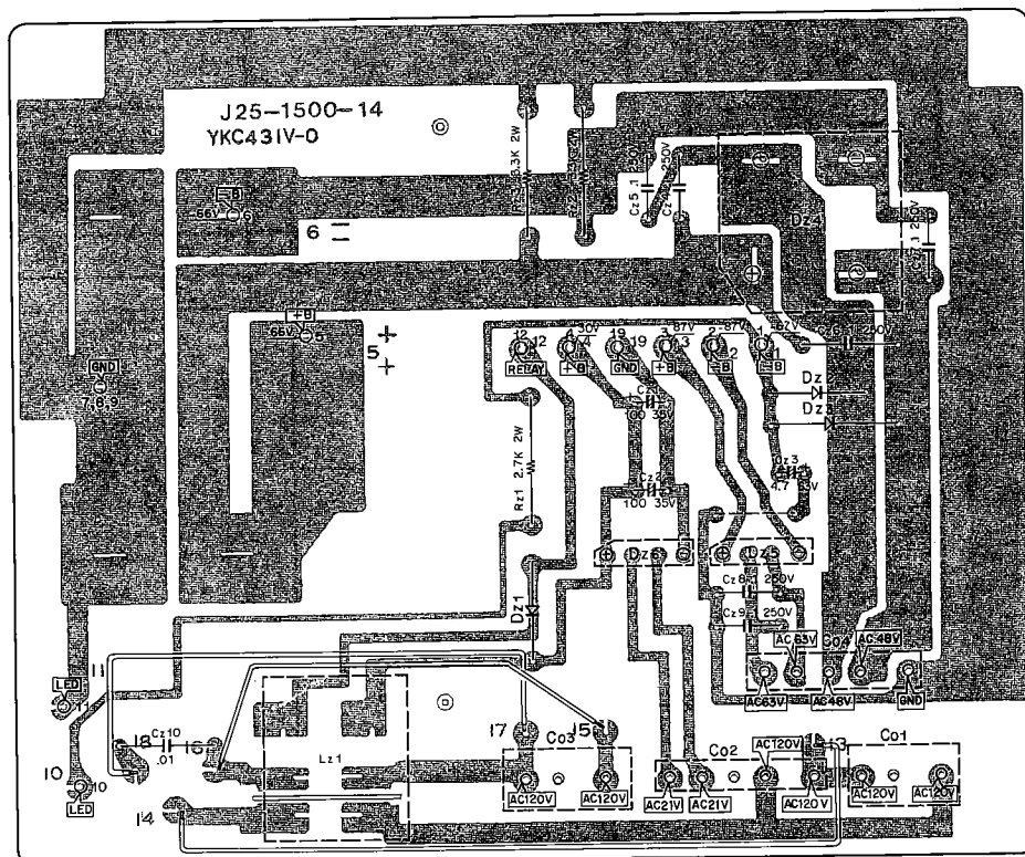
Dz1:V06B, Dz2, 3:V03C, Dz4:S25VB20, Dz5, 6:S1QB40
