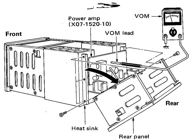
< The Way of Checking the Power Amp Unit >
