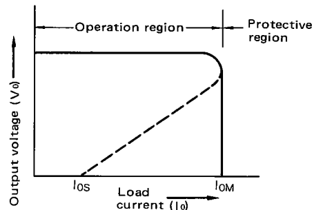
< Characteristics of Protection Circuit >
