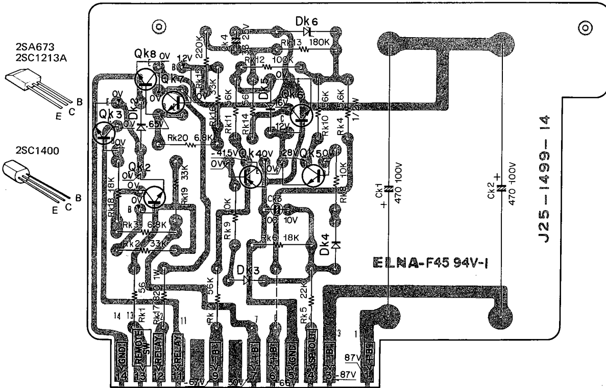
Qk2, 7:2SC1400(U), Qk3, 5, 6:2SC1213A (B) or (C), Qk4:2SA673A (B) or (C), Qk8:2SC1735 (D) or (E), Dk2:V06B, Dk3~5:1S2076A, Dk6:EQB01-28
