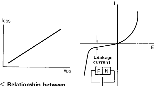
< I-E Characteristic of P-N Junction >
