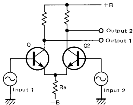
< Differential Amplifier >
