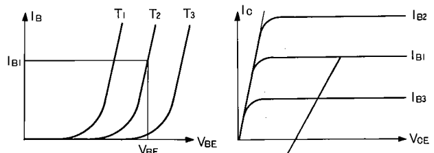
< V_{BE}-I_B Characteristics >
