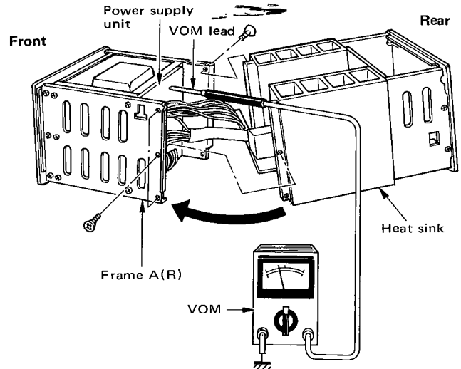
< The Way of Checking the Power Supply Unit >
