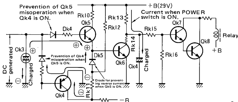
< Function of DC Protection Circuit >
