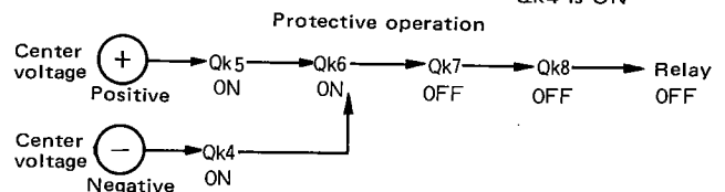
< Function of DC Protection Circuit >
