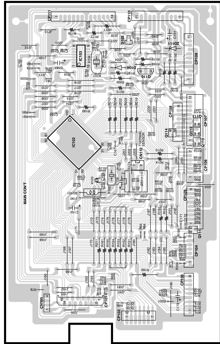
FRONT-3 BOARD
