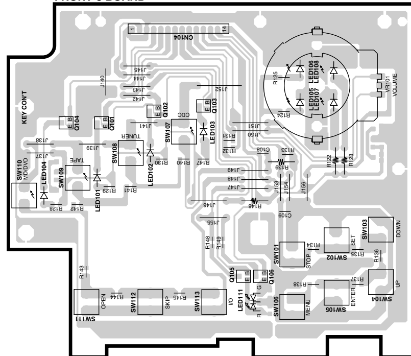
FRONT-3 BOARD
