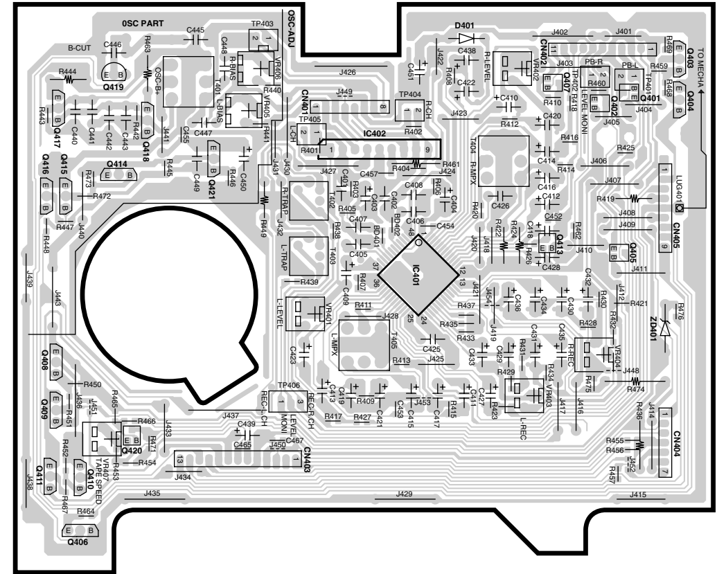
DECK BOARD
