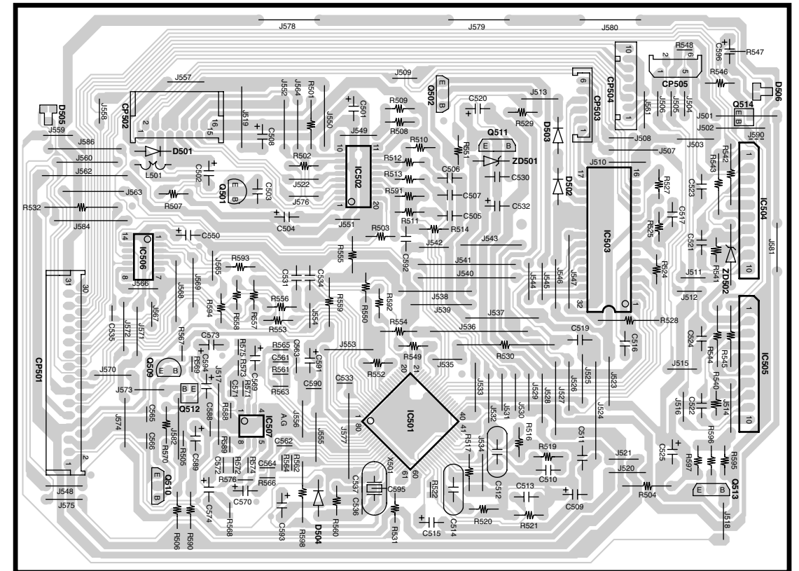
CD BOARD
