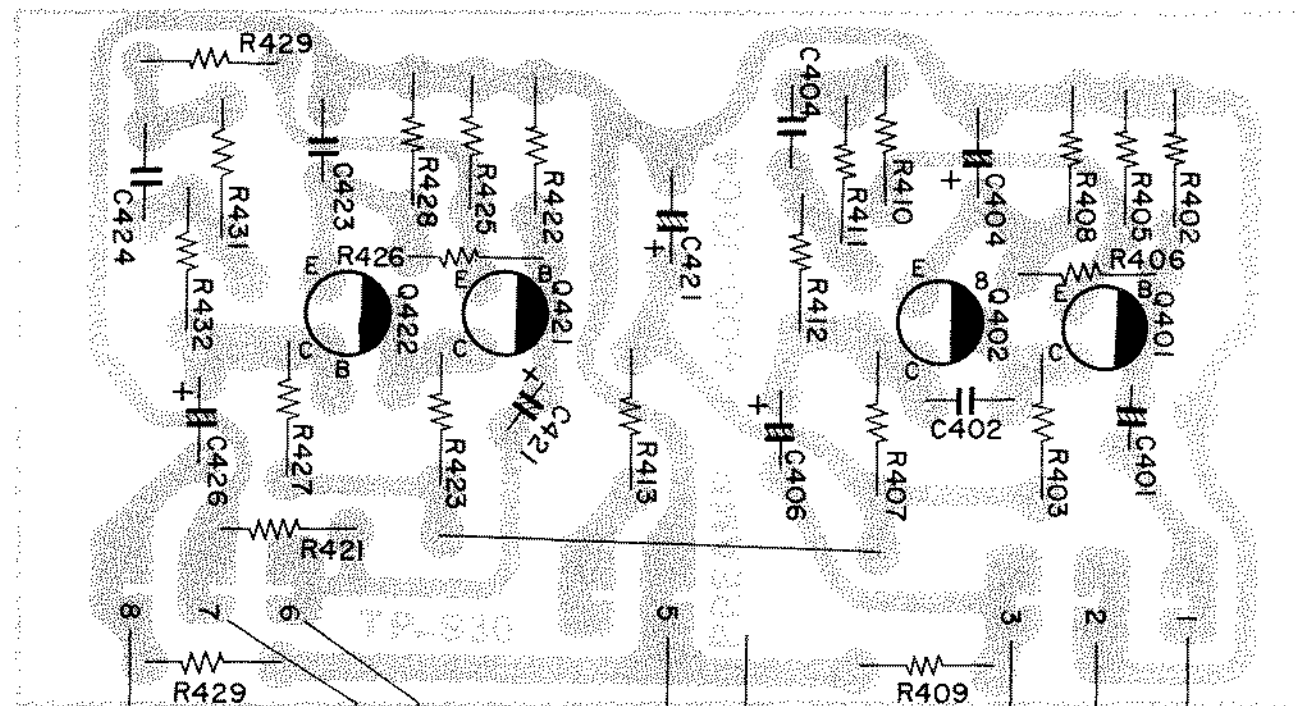
BOTTOM VIEW
