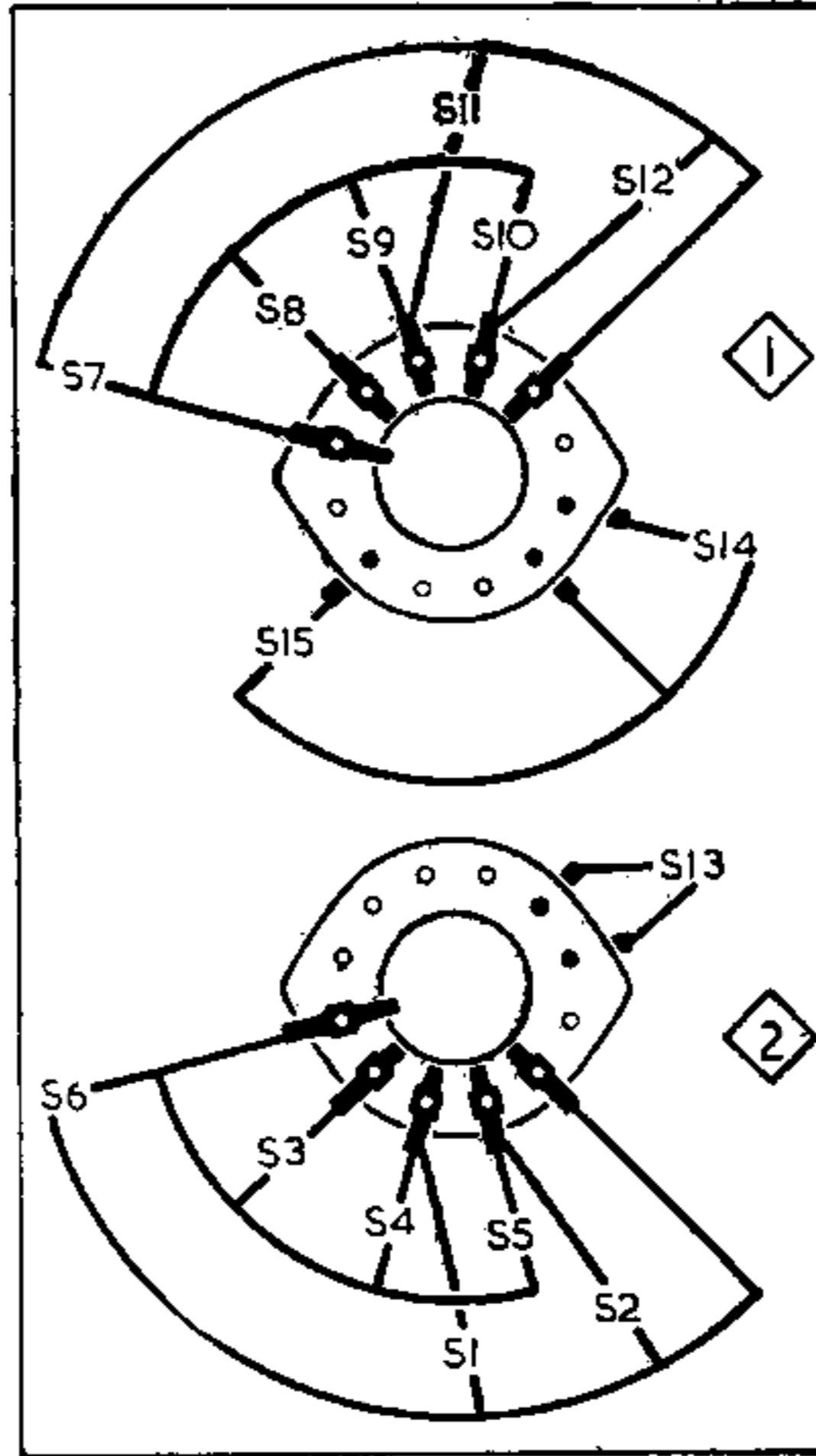
Diagrams of the waveband switch units, drawn as seen when viewed in the directions of the arrows in our underside view of the chassis. On the left is the associated switch table.
