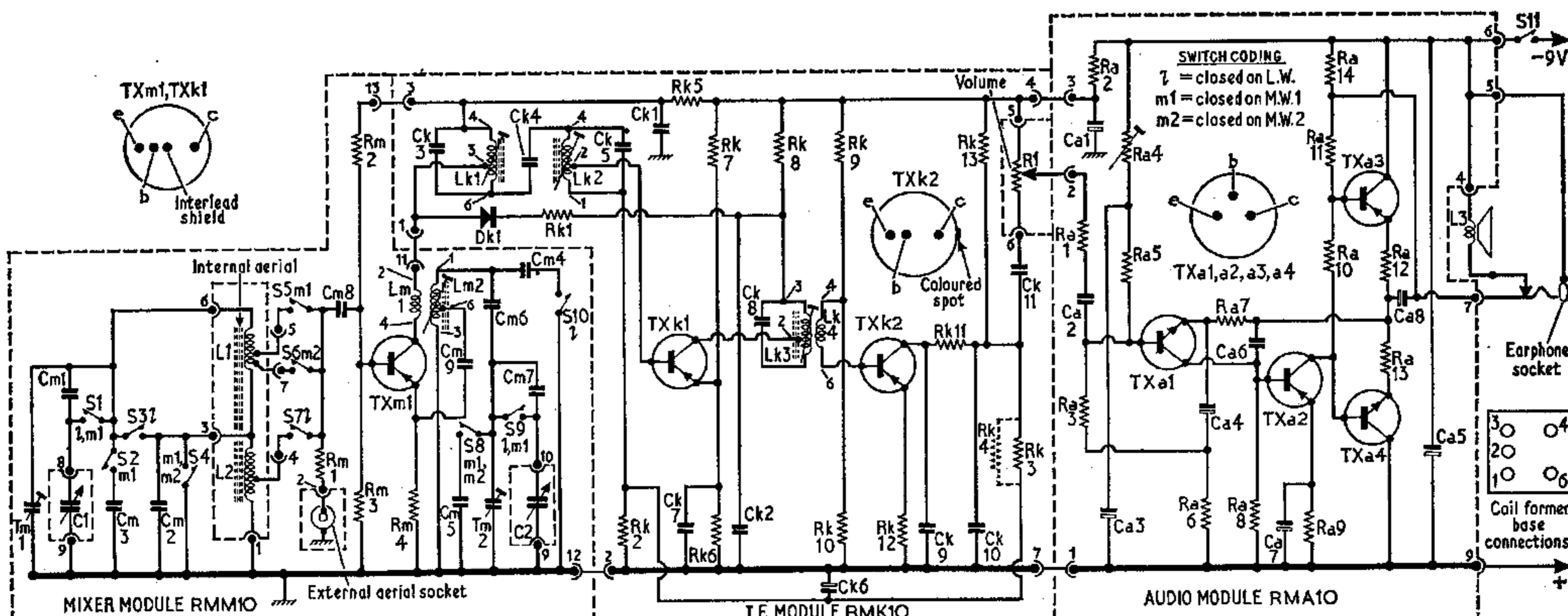
Circuit diagram of the KB KR021 and RGD RR221.
