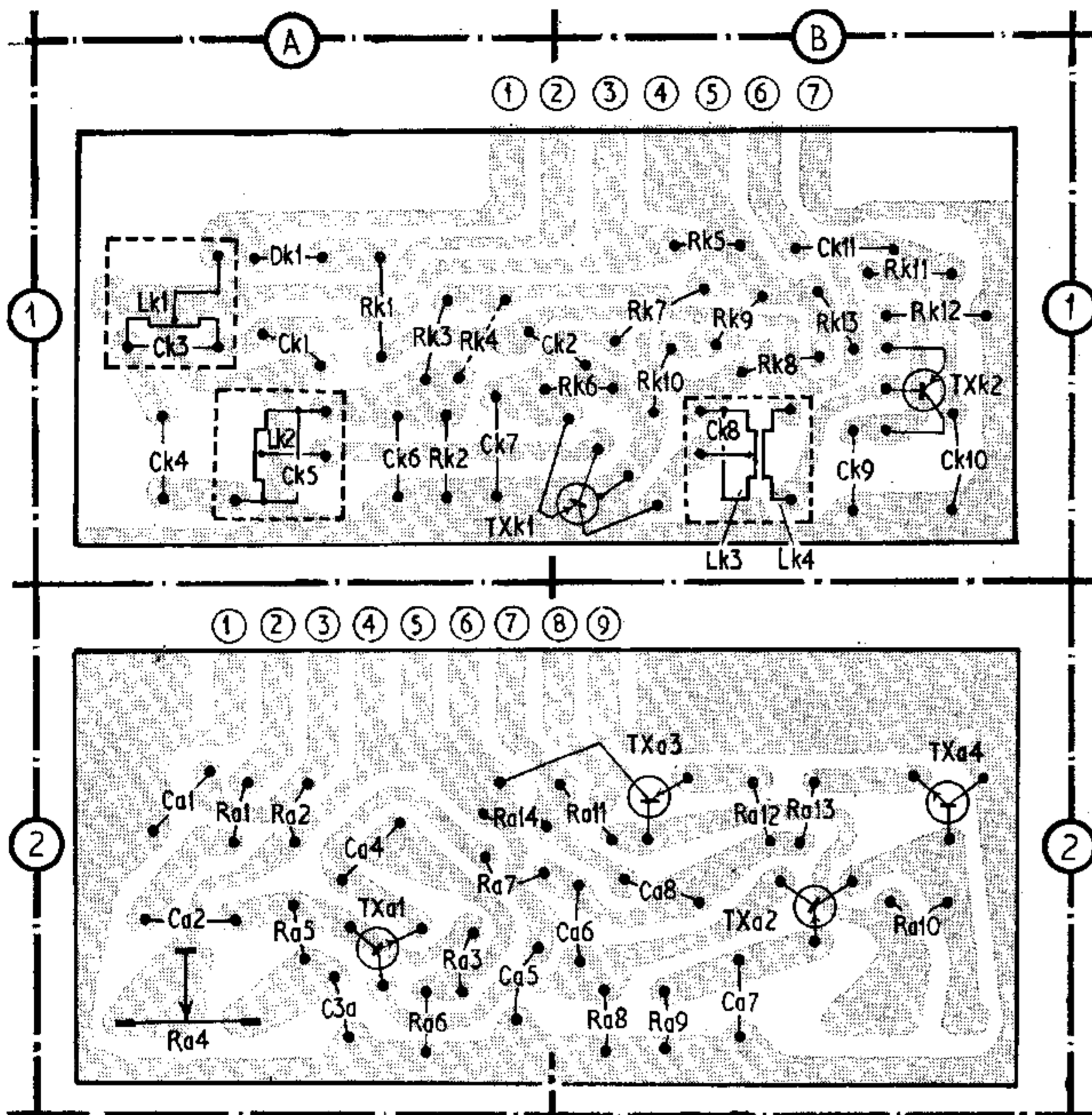
Above: The i.f. and a.f. printed panels.
