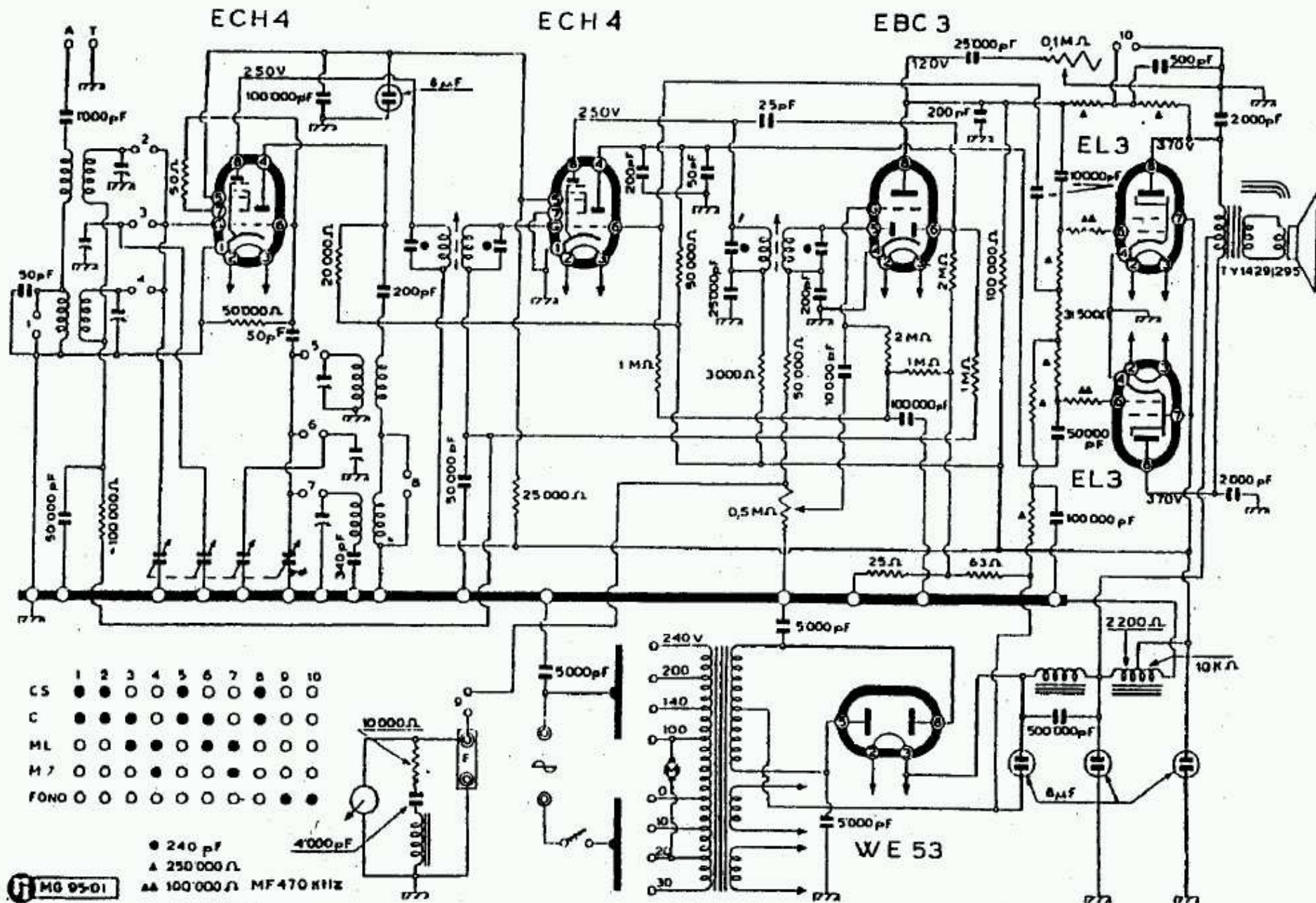
Kosmovox mod. 106 phono
