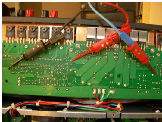
2 channel amplifier
