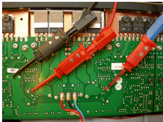
4 channel amplifier
