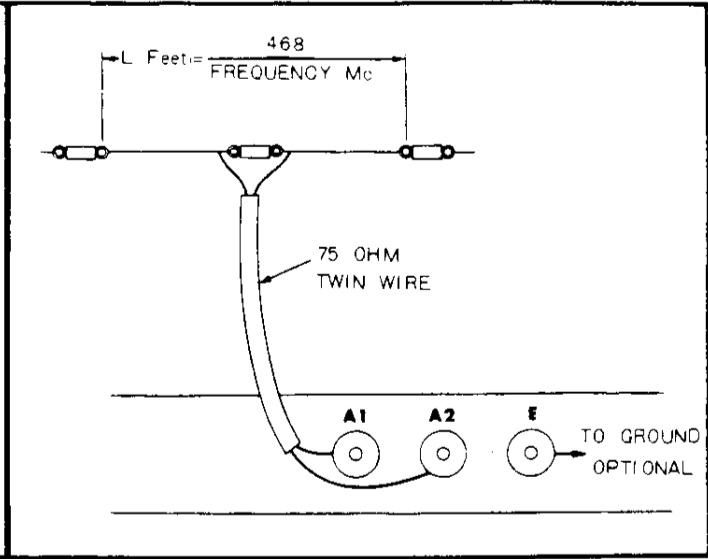
Figure 2. Doublet Antenna
