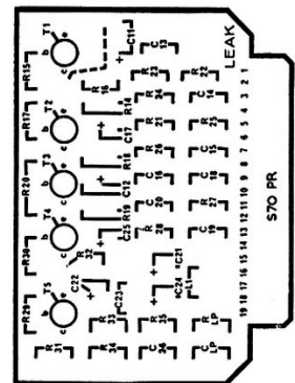
PRE-AMPLIFIER CIRCUIT BOARD LAYOUT DIAGRAM
