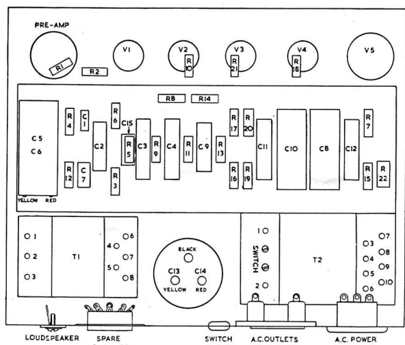
UNDER CHASSIS VIEW
