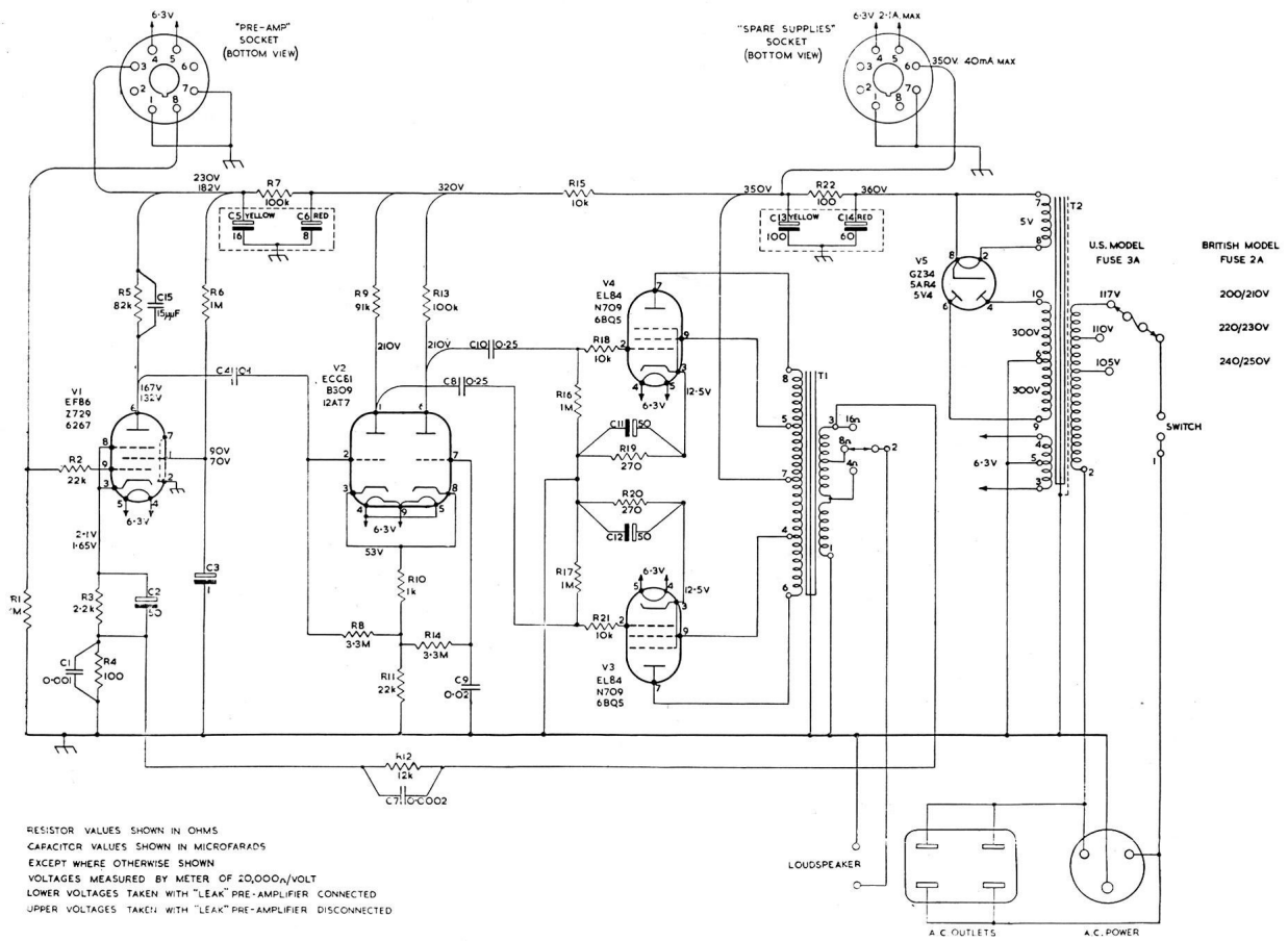
CIRCUIT DIAGRAM
