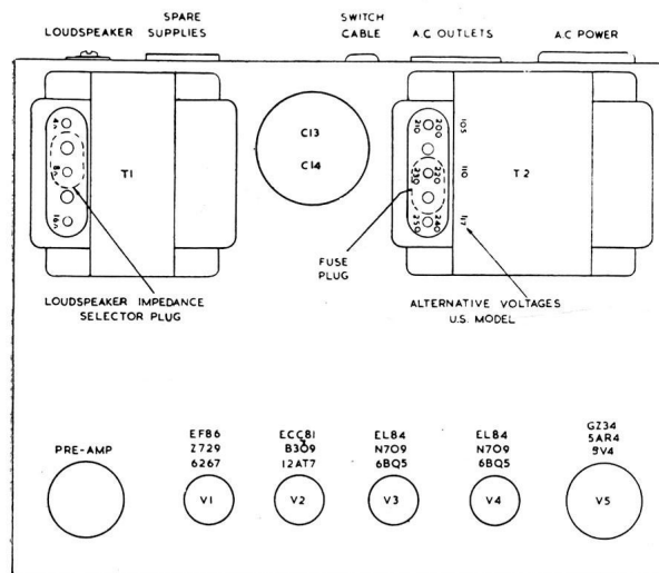
TOP CHASSIS VIEW
