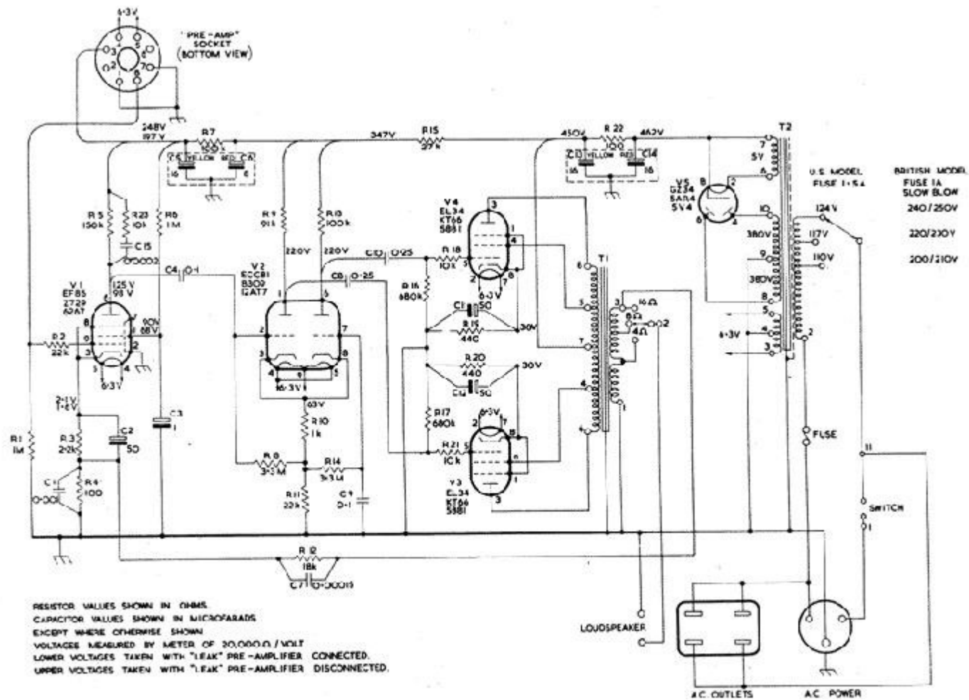
CIRCUIT DIAGRAM 'TL/25 PLUS' POWER AMPLIFIER
