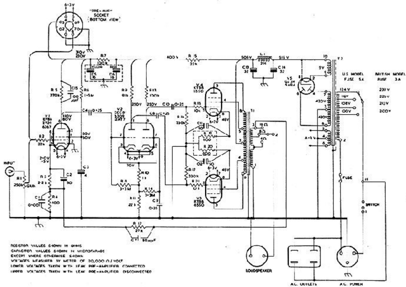
CIRCUIT DIAGRAM OF 'TL/50 PLUS' POWER AMPLIFIER
