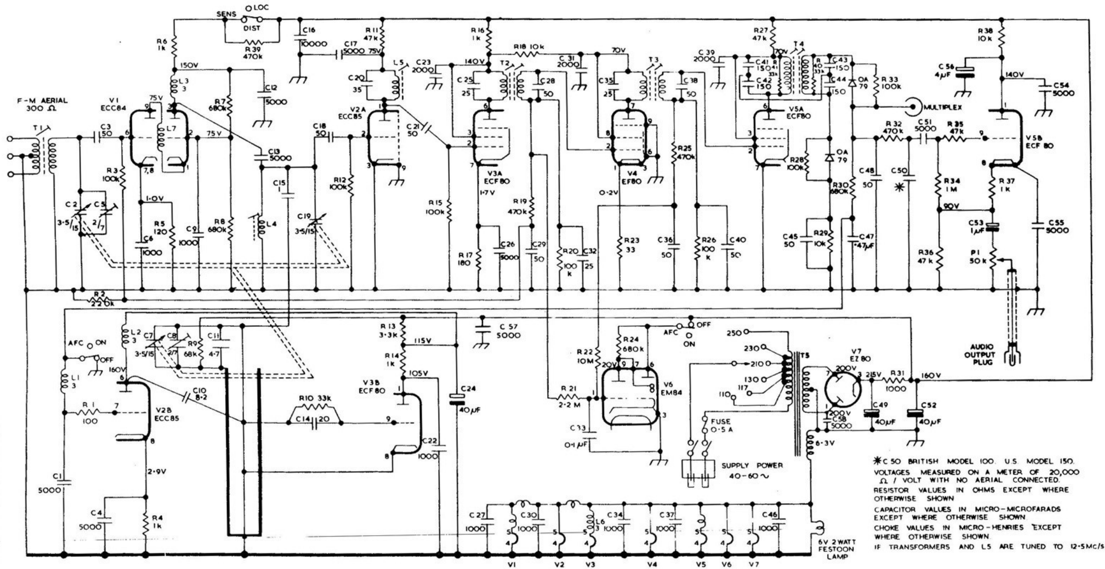
CIRCUIT DIAGRAM OF LEAK 'TROUG-LINE 3' F.M. TUNER
