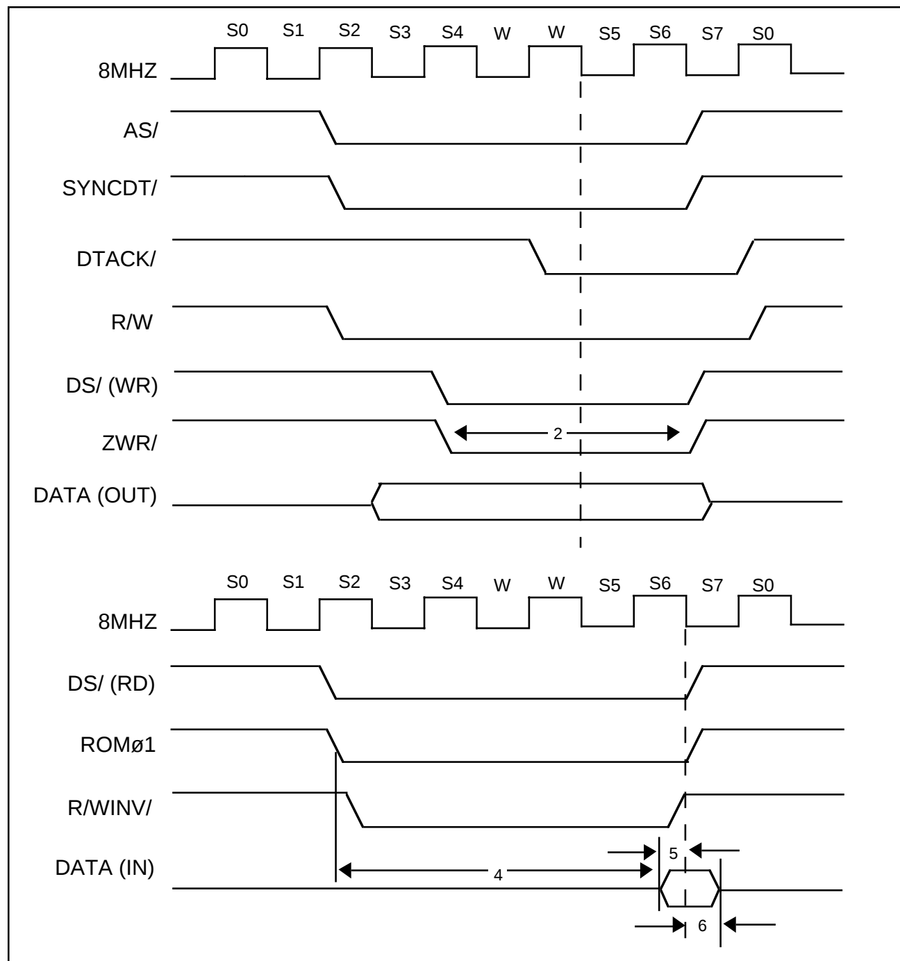
Synchronous Bus Timing
