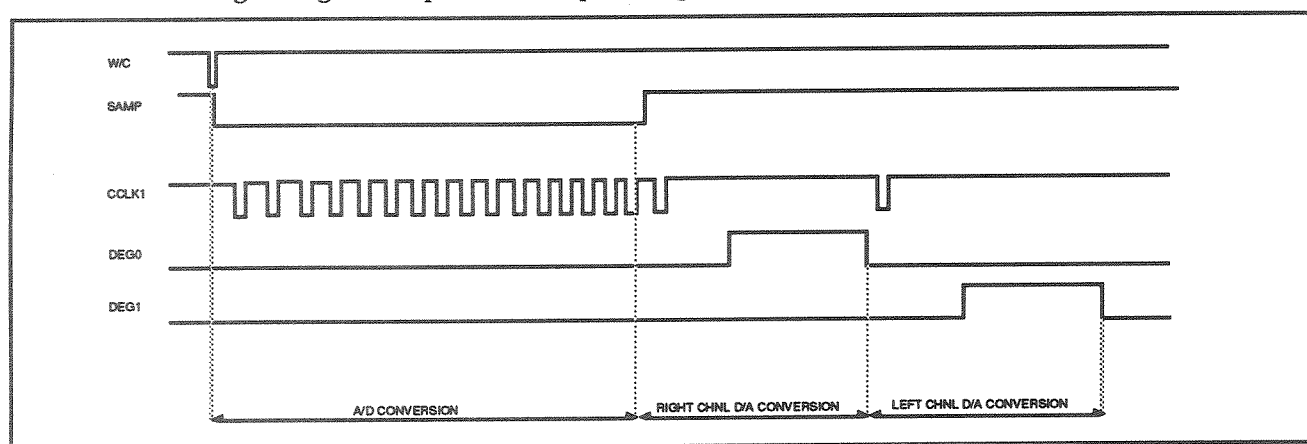
Converter Timing
