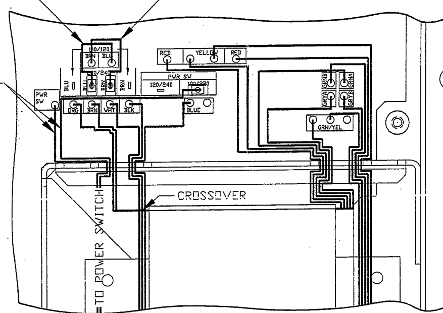
220 VOLTS SELECTION
