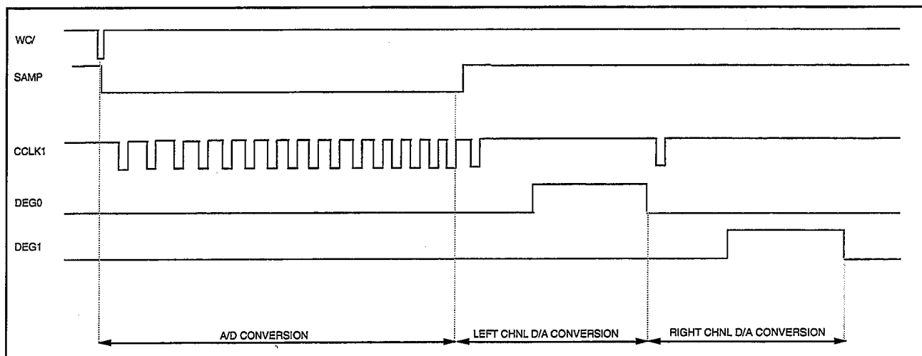
Converter Timing
