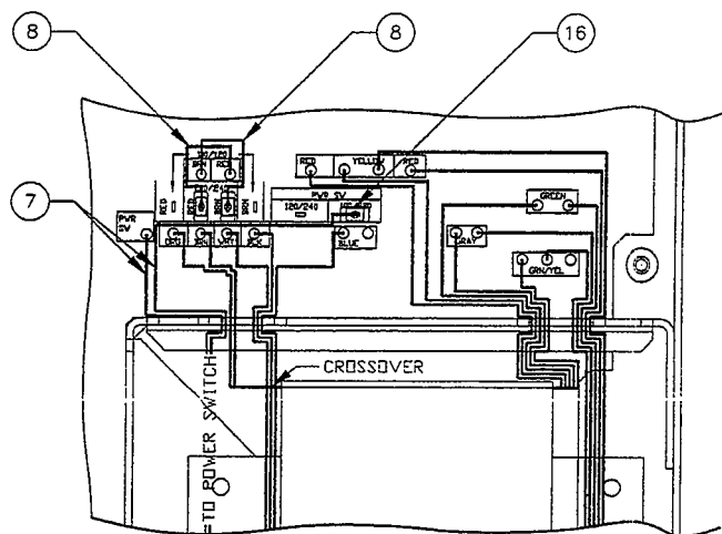
220 VOLTS SELECTION
