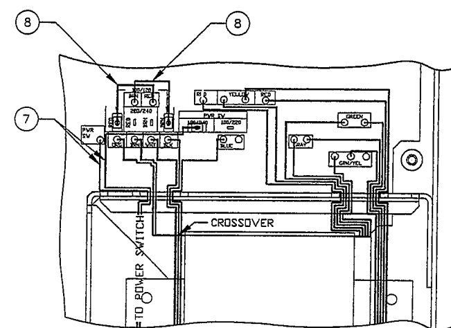
120 VOLTS SELECTION
