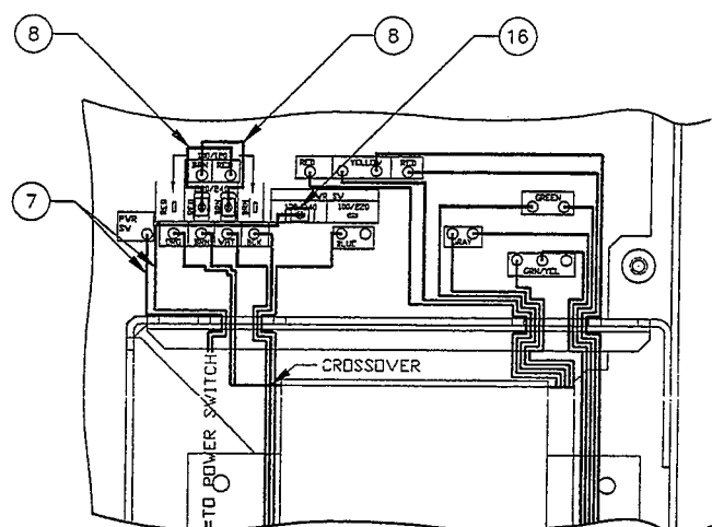
240 VOLTS SELECTION
