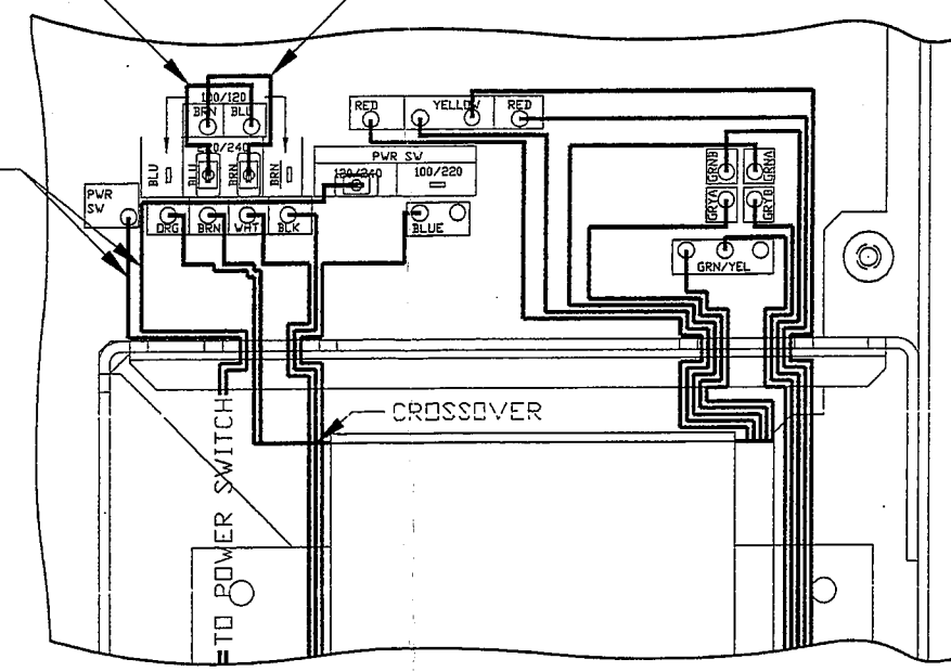
240 VOLTS SELECTION
