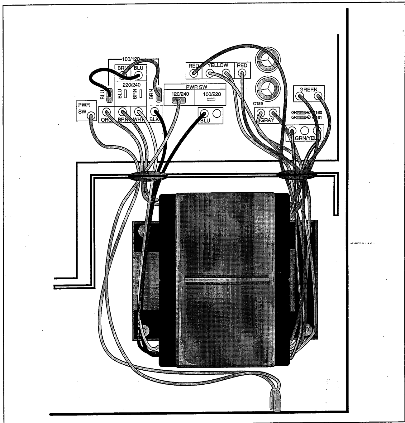
120VConnections
