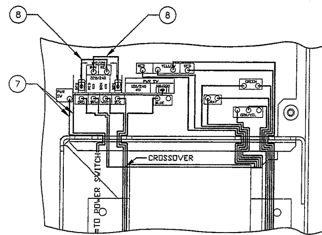
100 VOLTS SELECTION
