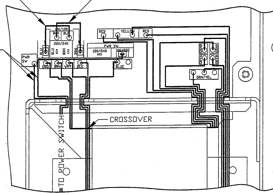
100 VOLTS SELECTION
