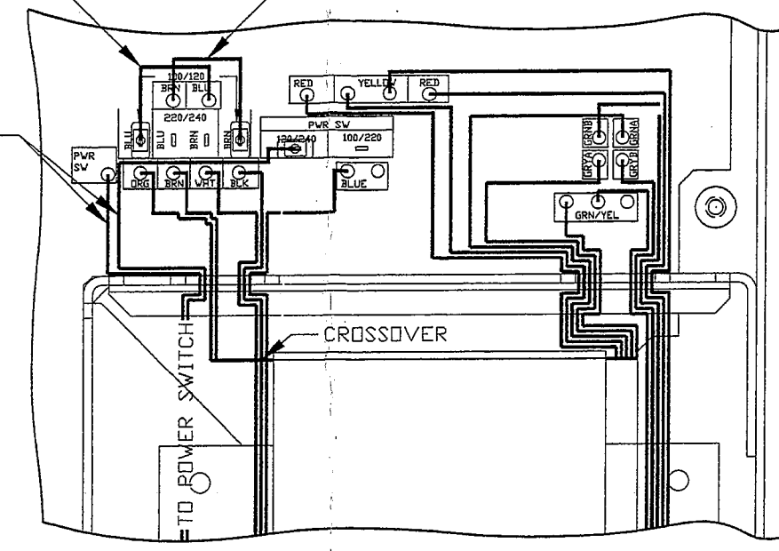
120 VOLTS SELECTION
