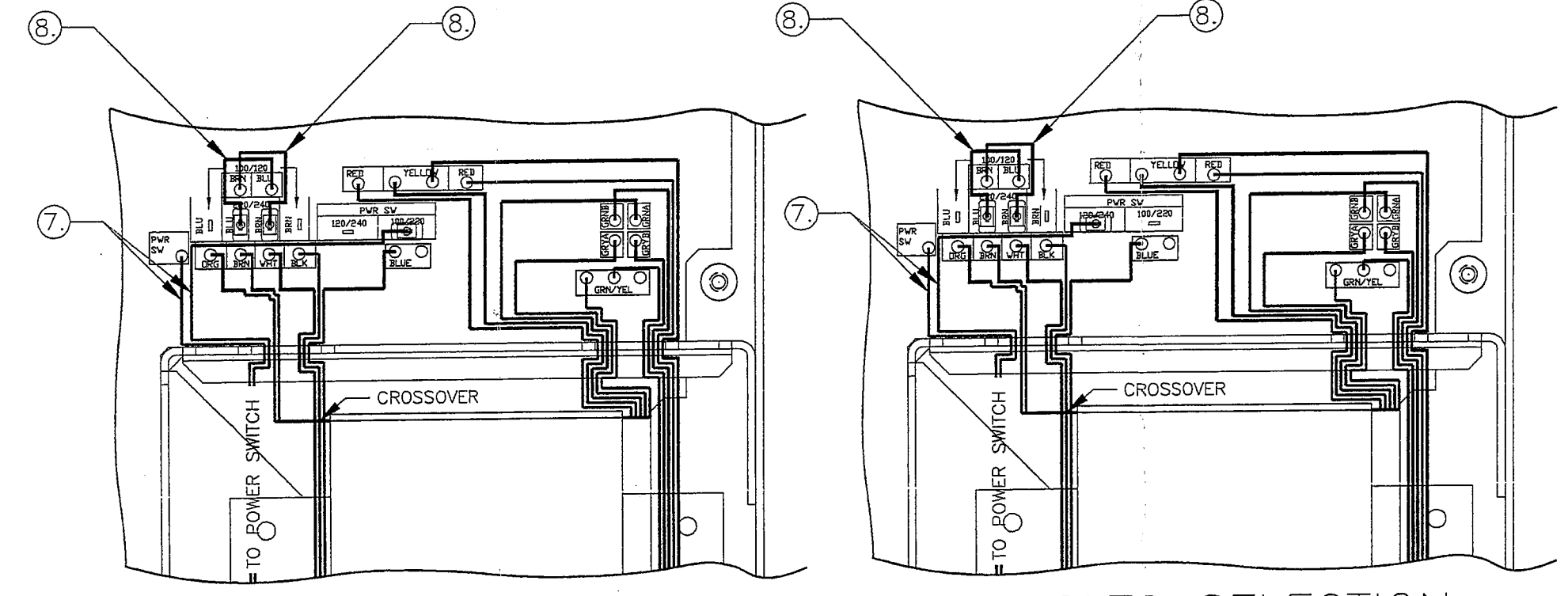
220 VOLTS SELECTION
