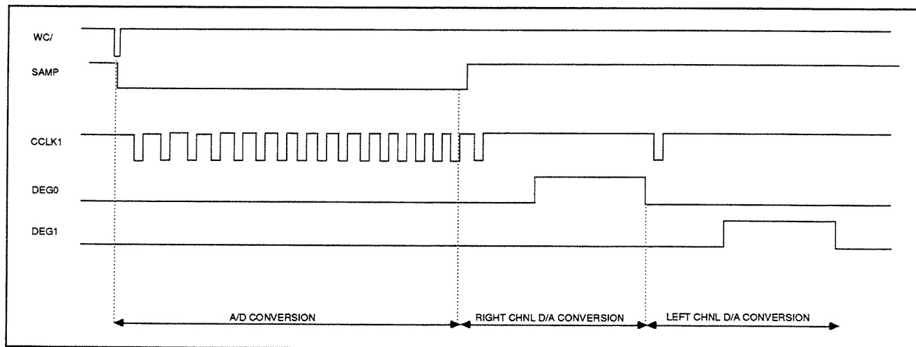
Converter Timing
