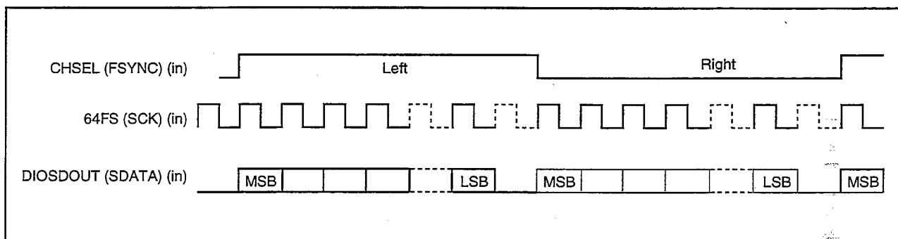
CS8402 Audio Serial Port Format
