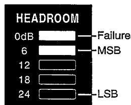
Binary Code 8 (1000)
