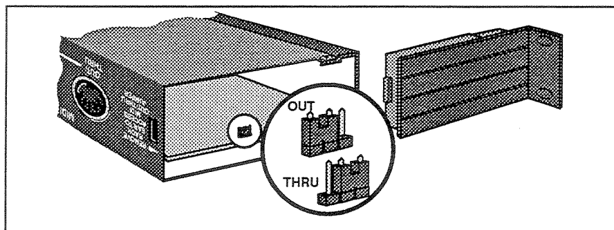
MIDI OUT/THRU Jumper
