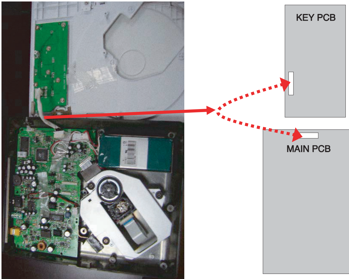
KEY PCB
