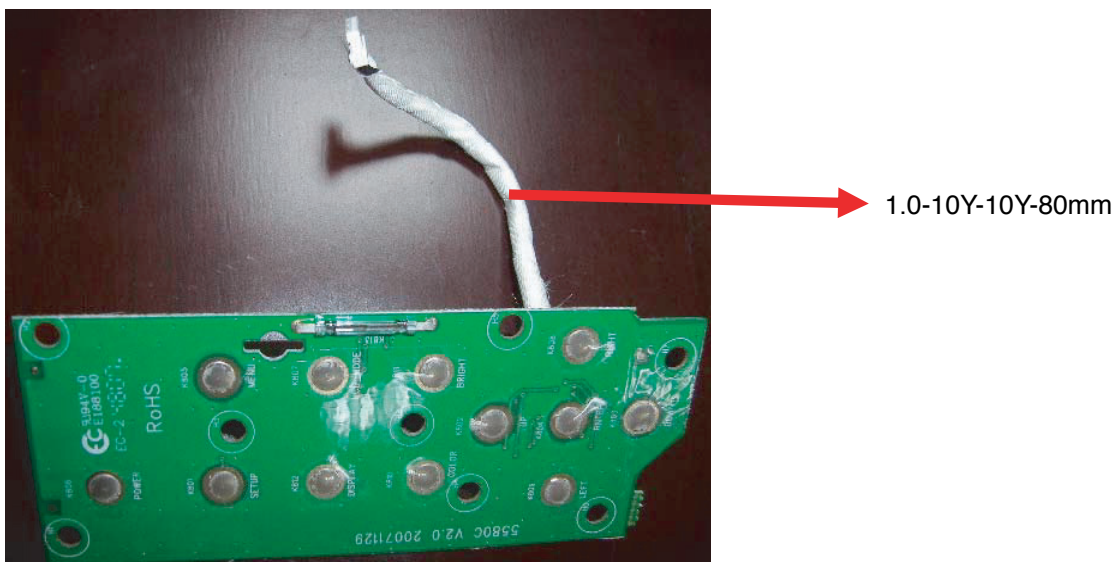
KEY PCB
