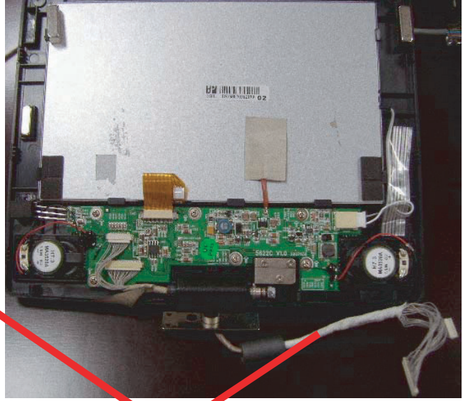
LCD PCB
