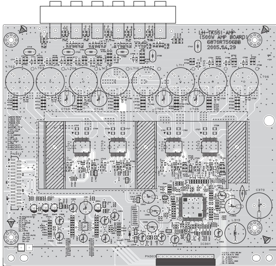
( TOP VIEW )
