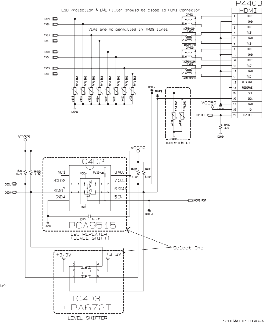
SCHEMATIC DIAGRAM (HDMI) LH-T9656 3854R11607A (#8)
