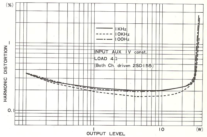
TOTAL HARMONIC DISTORTION (Both ch.)
