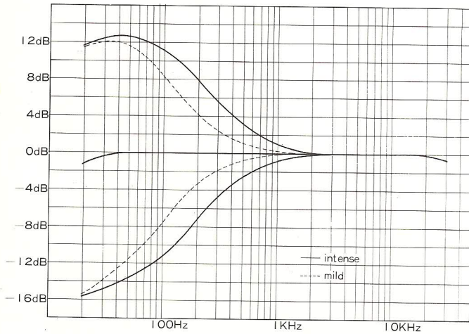
TREBLE FREQUENCY CONTROLS
