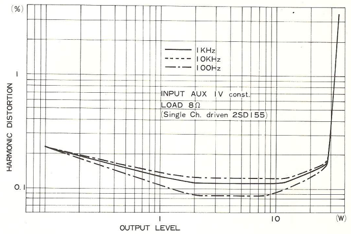
TOTAL HARMONIC DISTORTION (Single ch.)
