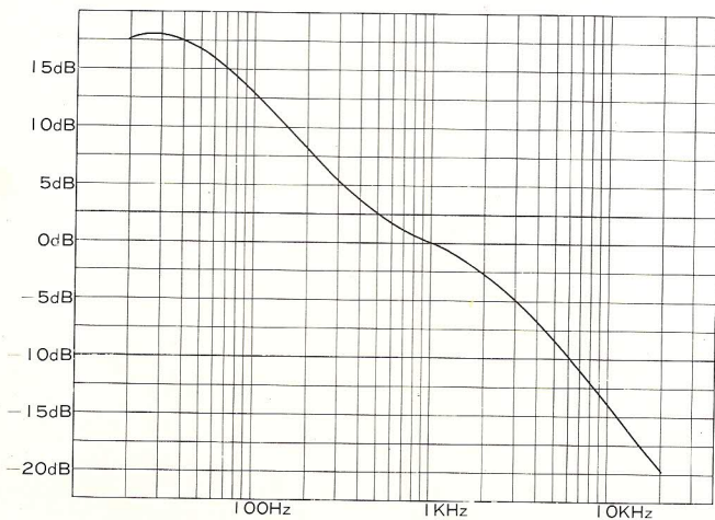
RIAA EQUALIZATION
