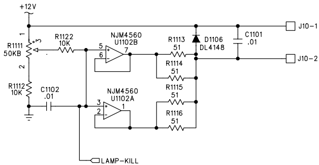
LAMP DIMMER
