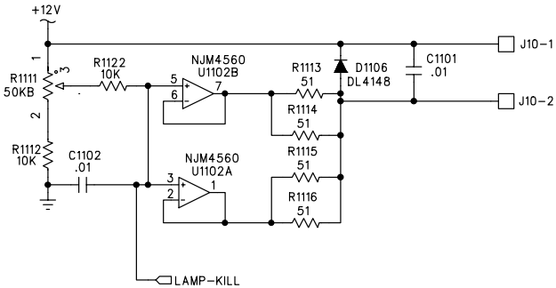
LAMP DIMMER
