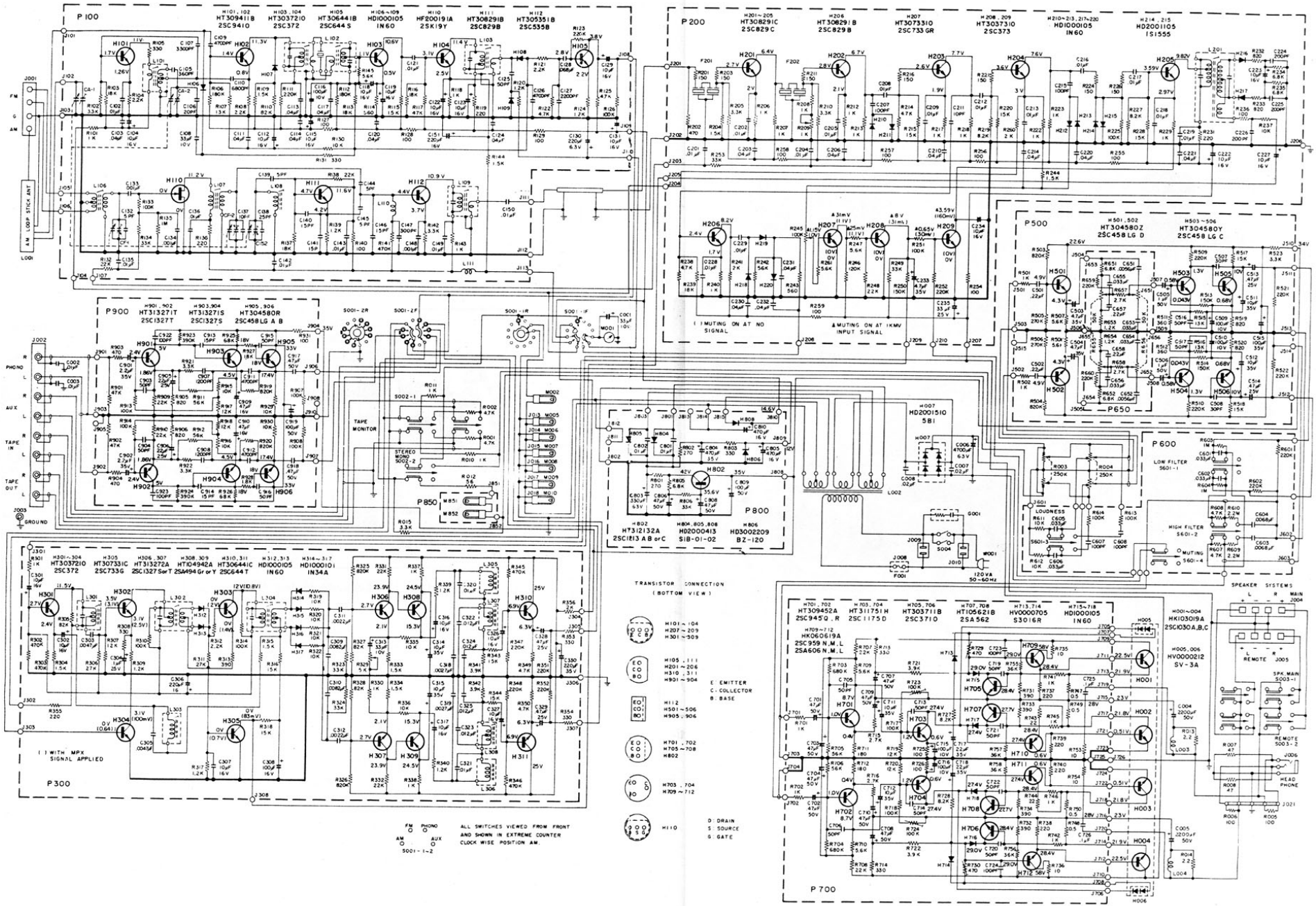
Figure 15. Schematic Diagram
