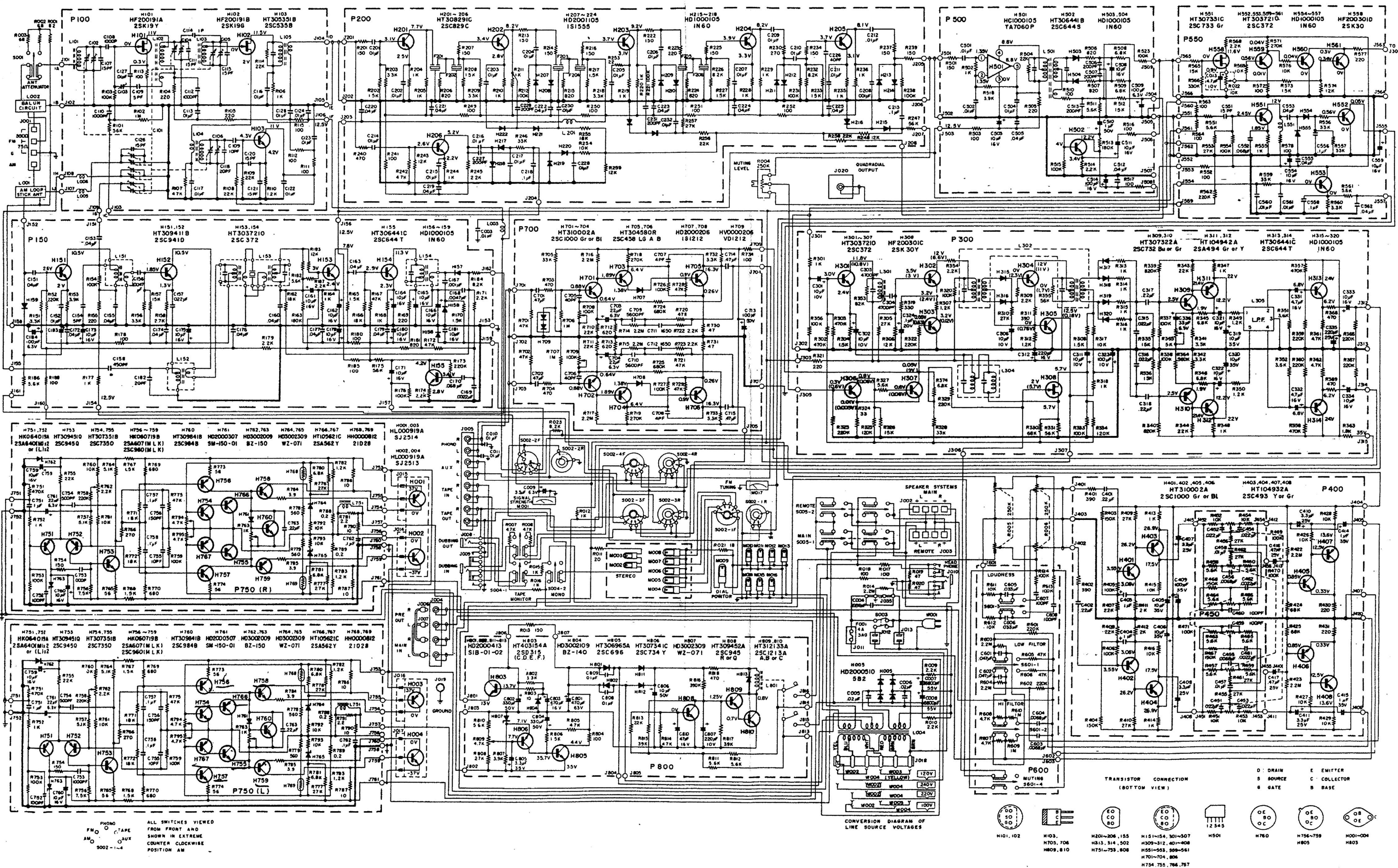
Figure 20. Schematic Diagram
