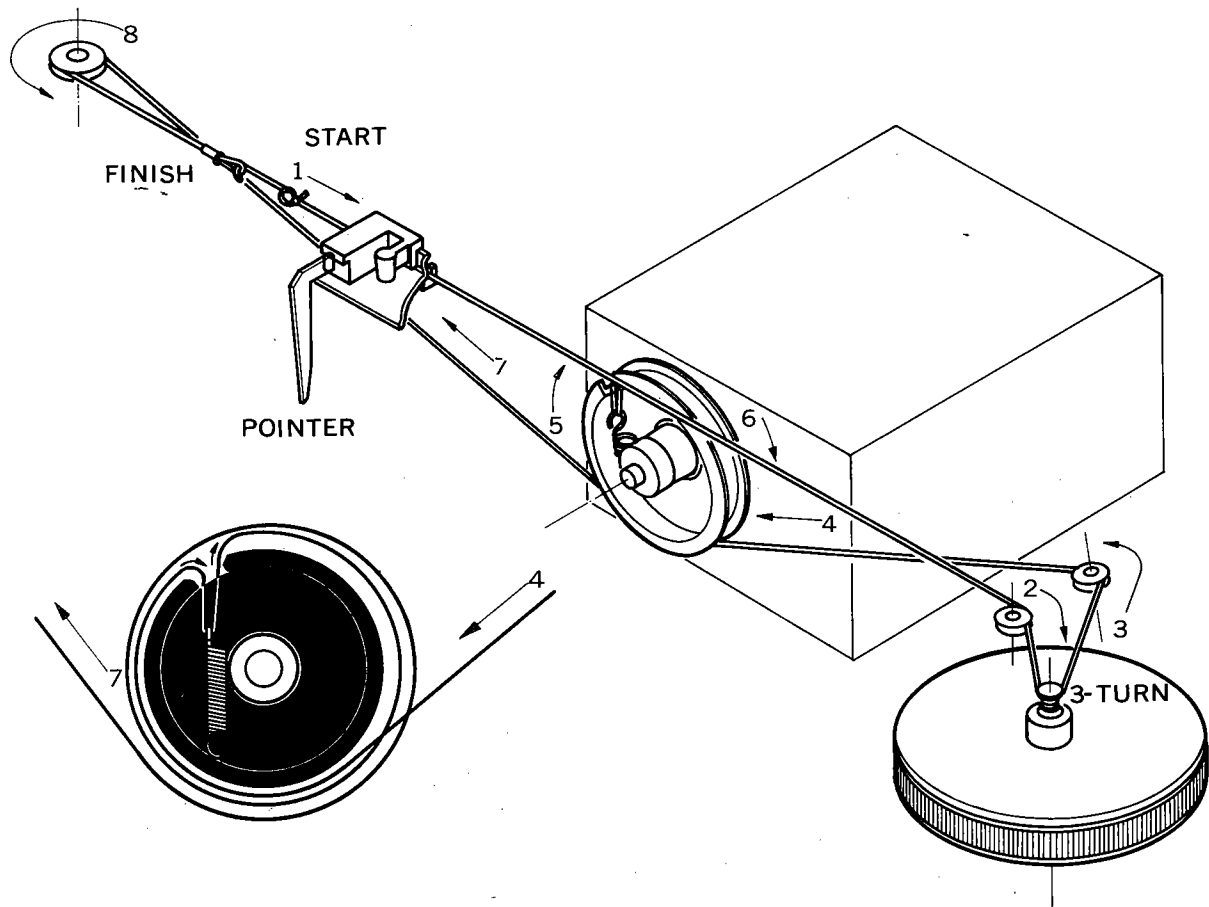
Figure 2. Dial Stringing
