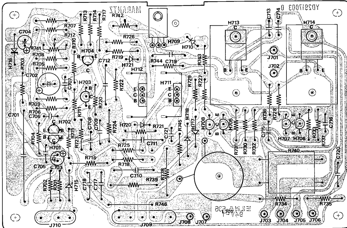
Figure 13. Power Amplifier Assembly P700 Component Locations
