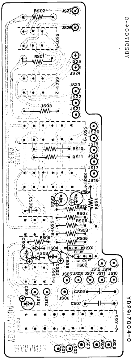
Figure 16. Dolby FM, Mono L, R, Multipath and Monitor Switches Assembly PS01 Component Locations
