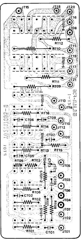
Figure 17. Muting, Speaker, Loudness, Power, Hi and Low Filter Switches PT01 Component Locations
