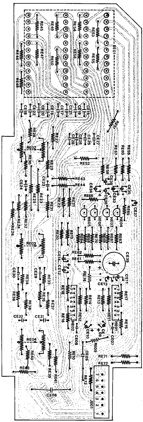
Figure 15. Pre and Tone Amplifier Assembly PE01 Component Locations
