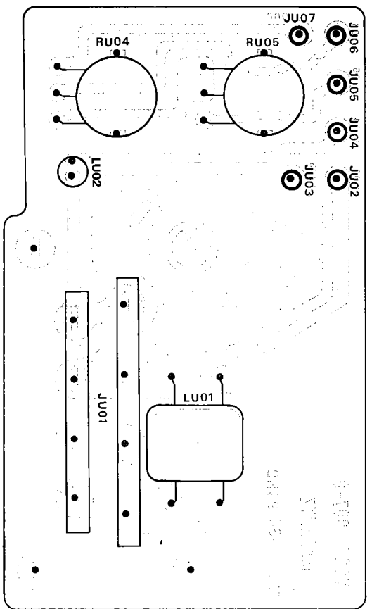
Figure 19. Muting Level and Antenna Attenuator Assembly PU01 Component Locations
