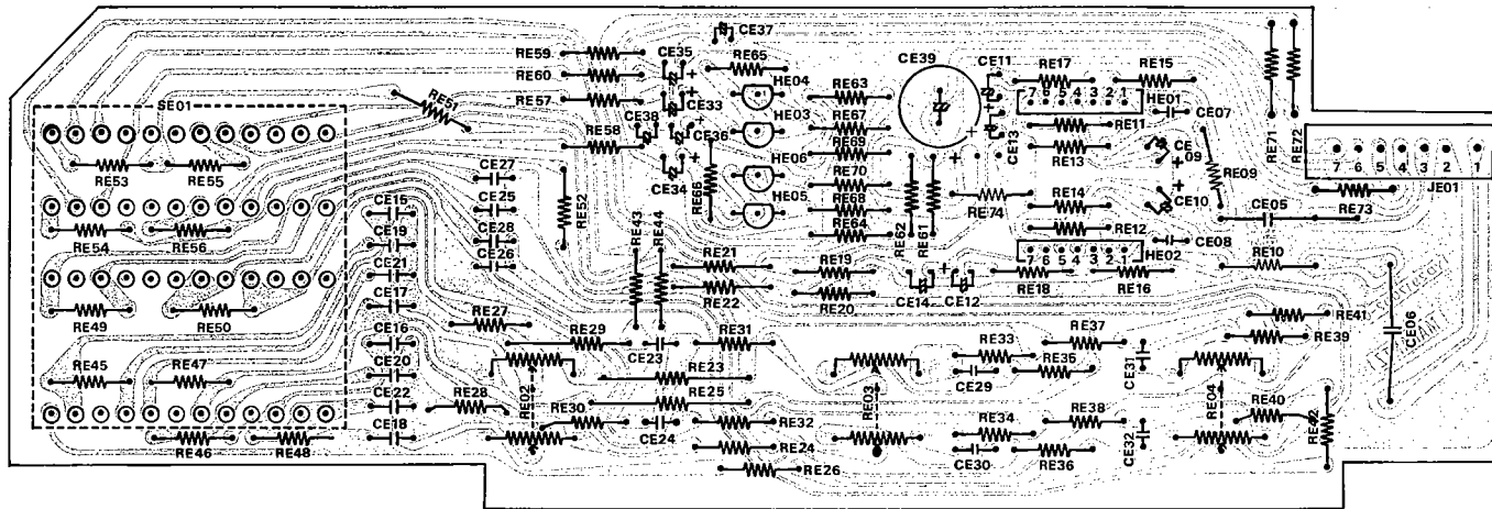
Figure 15. Pre and Tone Amplifier Assembly PE01 Component Locations
