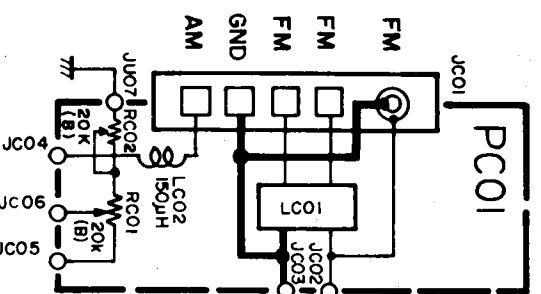
9.15 FM BALUN AND MUTING LEVEL CIRCUIT BOARD PC01
